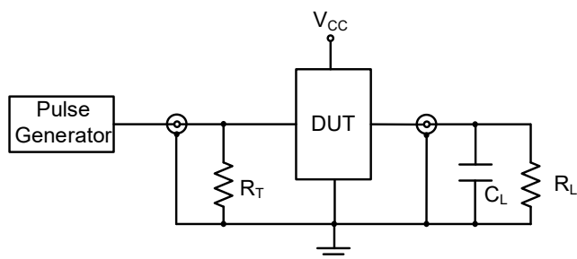
Figure4. Test Circuit
