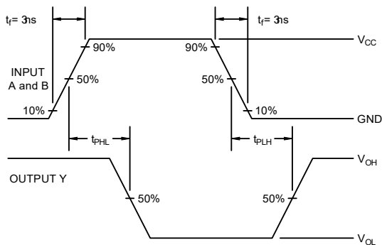
Figure3. Switching Waveform
