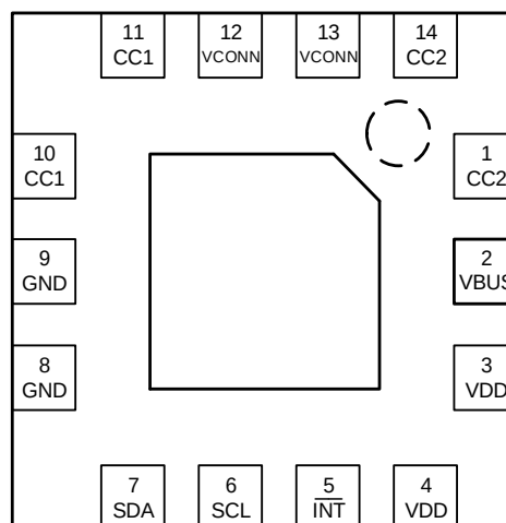
BOOTM VIEW
