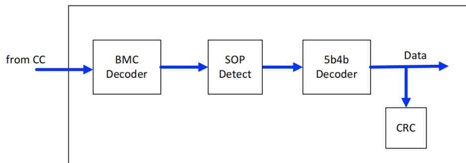
Figure 8. ET7304 BMC Receiver Block Diagram
