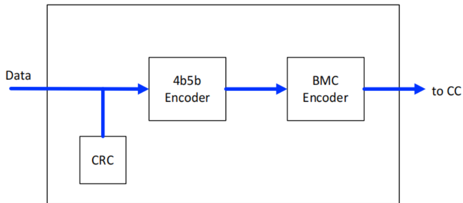
Figure 7. ET7304 BMC Transmitter Block Diagram
