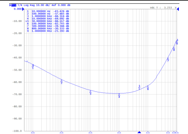
PSRR VS Output Current( I_{OUT}=150\text{mA} )
