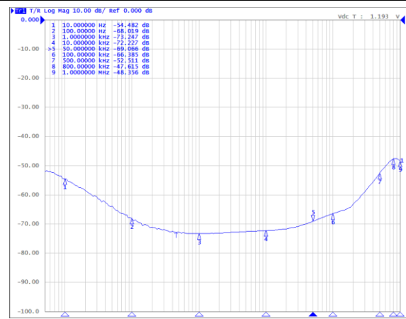
PSRR VS Output Current( I_{OUT}=150mA )
