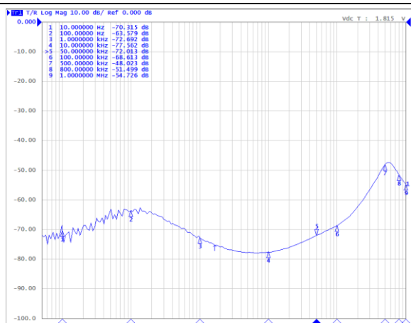
PSRR VS Output Current(I OUT =30mA)
