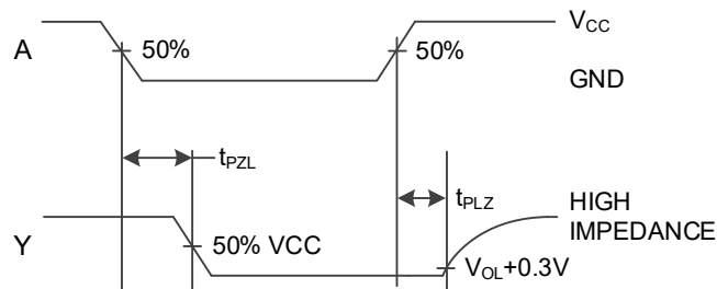
Figure3. Switching Waveform
