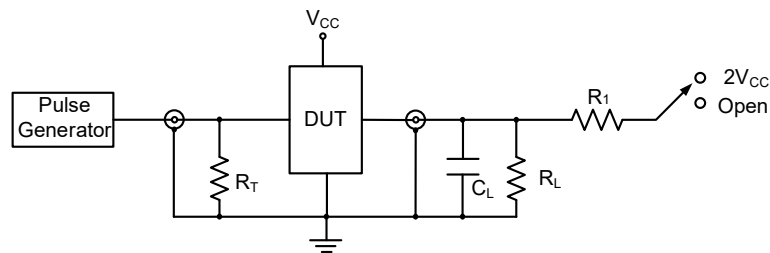
Figure4. Test Circuit R_T = 50\Omega(\text{Typ})
