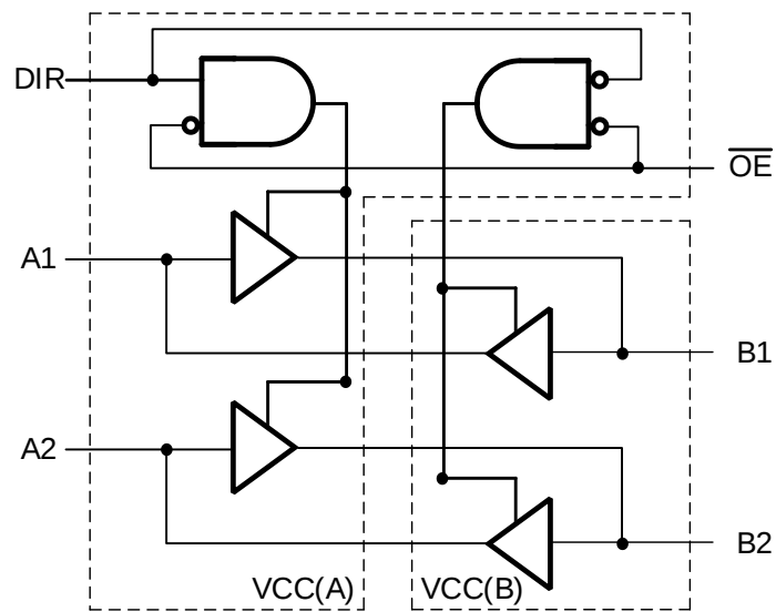
Figure3. Logic Diagram
