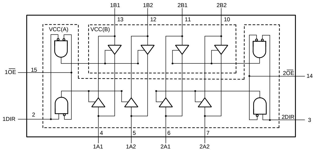
Figure2. Logic Symbol
