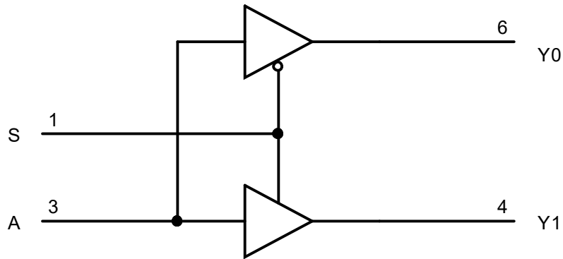
Figure2. Logic Symbol
