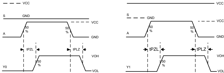
Figure3. Switching Waveform
