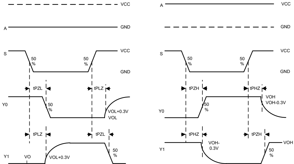
Figure6. Output Enable/Disable Waveform
