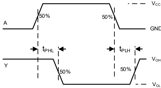
Figure3. Switching Waveform
