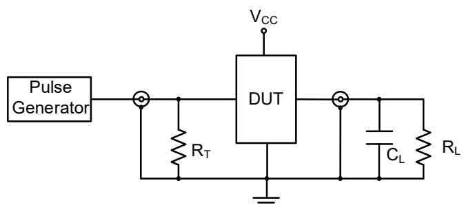
Figure4. Test Circuit
