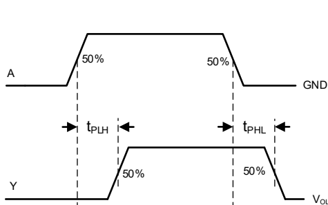
Figure3. Switching Waveform
