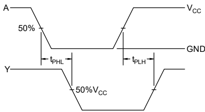
Figure3. Switching Waveform
