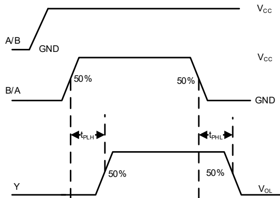
Figure3. Switching Waveform
