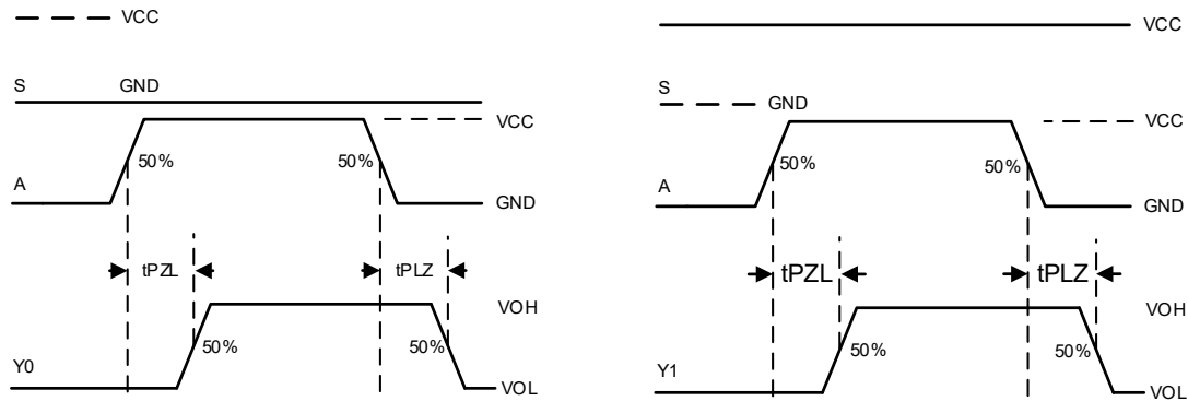
Figure3. Switching Waveform
