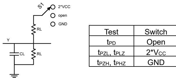
Figure6. Output Enable/Disable Time Test Circuit
