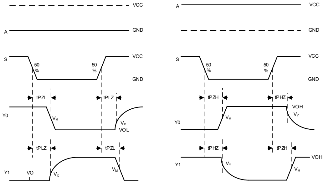
Figure5. Output Enable/Disable Waveform
