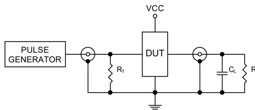
Figure4. Test Circuit R_T = 50\Omega(\text{typ})
