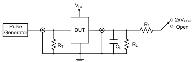
Figure4. Test Circuit
