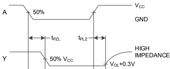
Figure3. Switching Waveform
