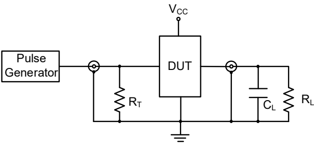
Figure4. Test Circuit
