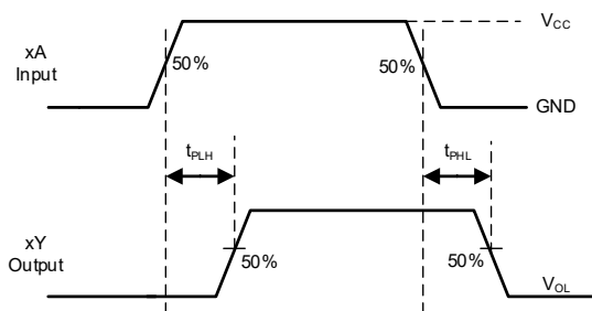
Figure3. Switching Waveform
