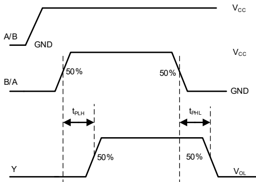
Figure3. Switching Waveform
