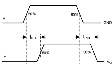
Figure3. Switching Waveform
