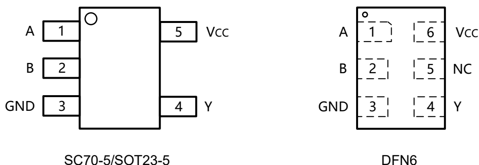
Figure1. Pin Configuration
