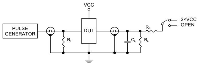
Figure4. Test Circuit R_T = 50\Omega(\text{Typ})
