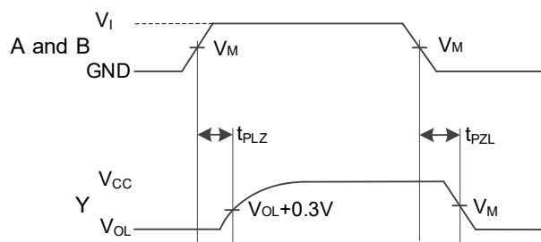
Figure3. Switching Waveforms
