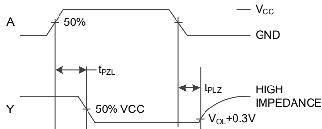
Figure3. Switching Waveforms
