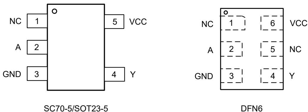
Figure1. Pin Configuration
