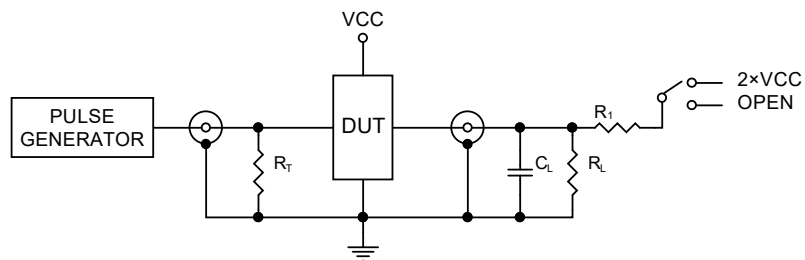
Figure4. Test Circuit R_T = 50\Omega (Typ)
