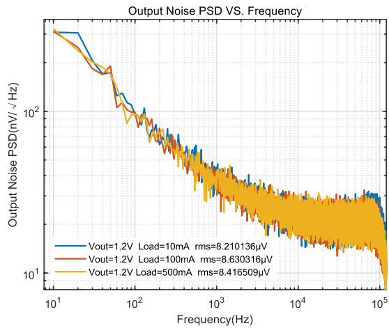
Output Noise PSD
