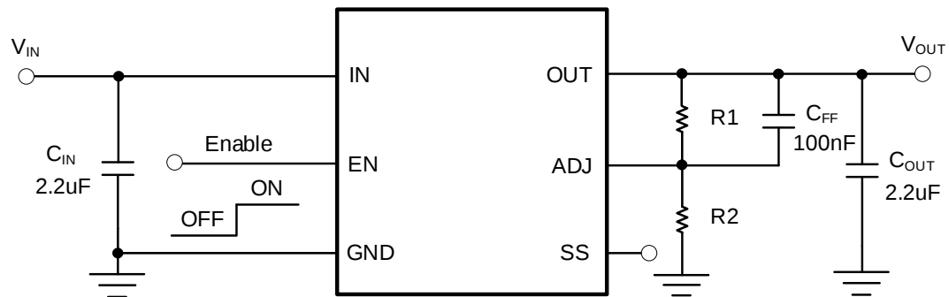
ET55HS24ADJ with Adjustable Output Voltage Circuit
