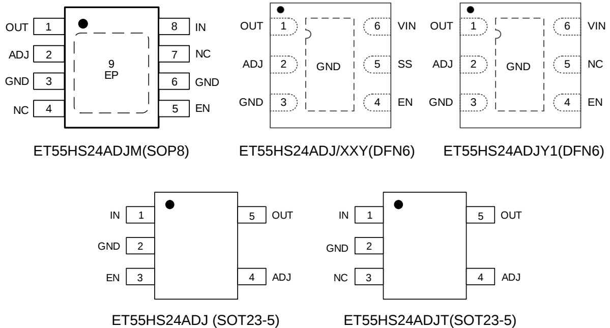
Figure1. Pin Configuration
