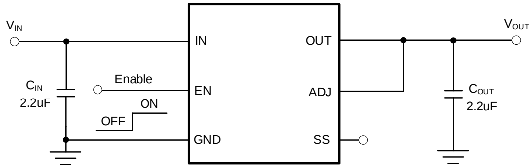
ET55HS24XXY with Fixed Output Voltage Circuit
