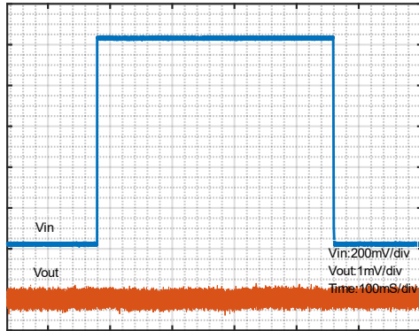
Line Transient
