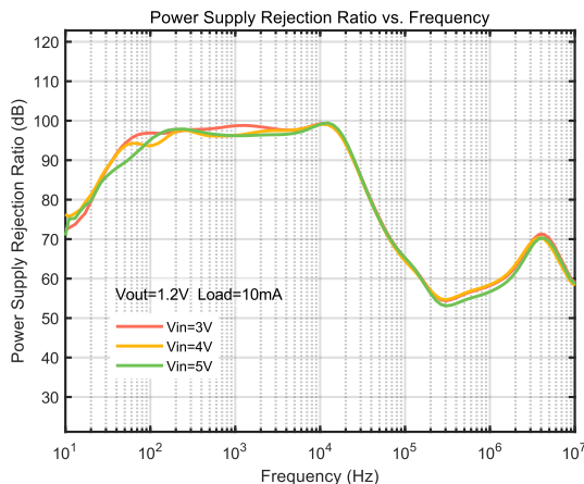
PSRR( I_{OUT} = 10mA )
