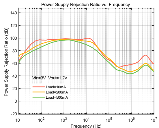
PSRR( V_{IN} = 3V )
