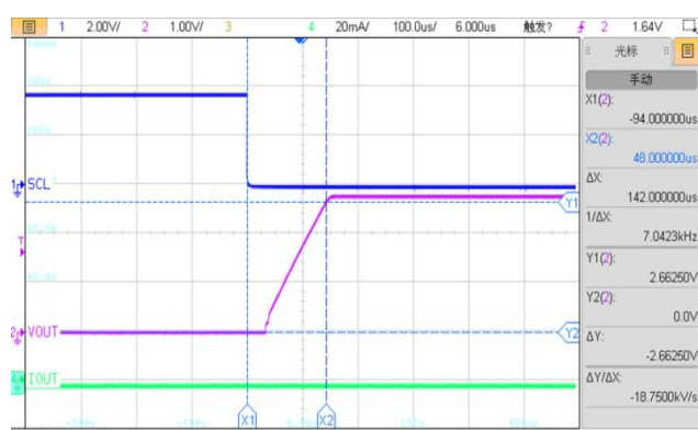
LDO3/4/5/6/7 Ton
