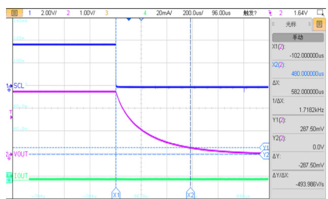
LDO3/4/5/6/7 Toff
