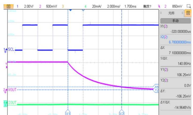
LDO1/2 Toff
