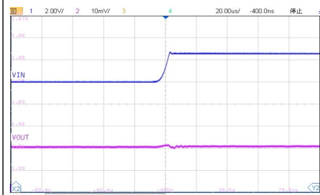
Line Transient Response V_{IN} = 2.8V \sim 5.5V , V_{OUT} = 1.8V , I_{OUT} = 1mA
