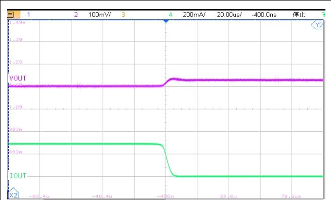
Load Transient Response V_{IN} = 2.2V , V_{OUT} = 1.2V , I_{OUT} = 300mA \sim 1mA
