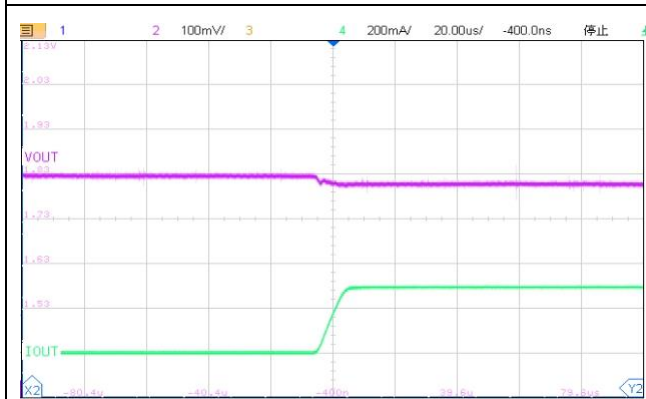
Load Transient Response V_{IN} = 2.8V , V_{OUT} = 1.8V , I_{OUT} = 1mA \sim 300mA
