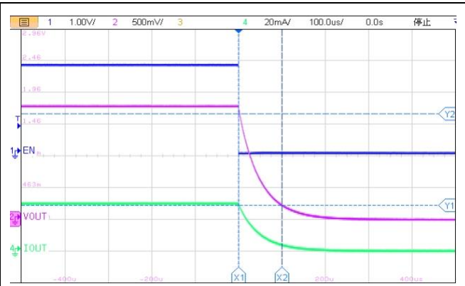
Turn Off Speed VS EN Voltage ( I_{OUT} = 30mA )
