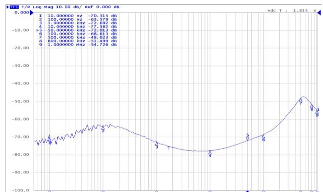
PSRR VS Output Current ( I_{OUT} = 10mA )
