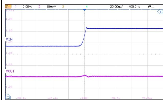
Line Transient Response V_{IN} = 2.2V \sim 5.5V , V_{OUT} = 1.2V , I_{OUT} = 1mA
