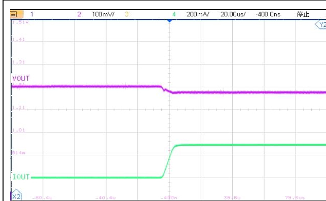
Load Transient Response V_{IN} = 2.2V , V_{OUT} = 1.2V , I_{OUT} = 1mA \sim 300mA
