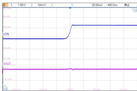
Line Transient Response V_{IN} = 4.3V \sim 5.5V , V_{OUT} = 3.3V , I_{OUT} = 1mA
