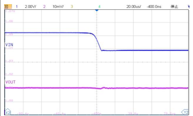
Line Transient Response V_{IN} = 5.5V \sim 2.8V , V_{OUT} = 1.8V , I_{OUT} = 1mA
