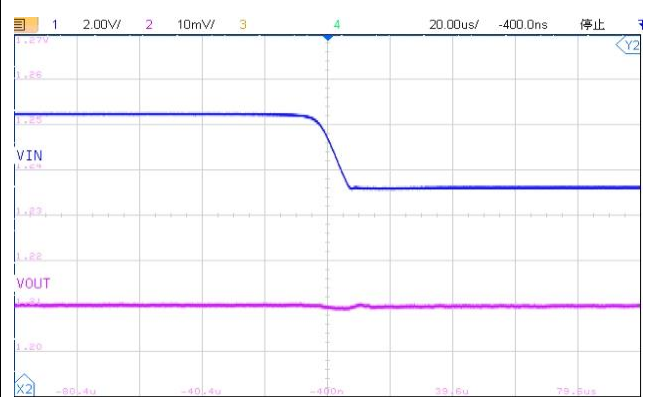
Line Transient Response V_{IN} = 5.5V \sim 2.2V , V_{OUT} = 1.2V , I_{OUT} = 1mA
