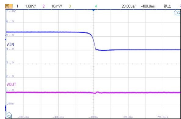
Line Transient Response V_{IN} = 5.5V \sim 4.3V , V_{OUT} = 3.3V , I_{OUT} = 1mA
