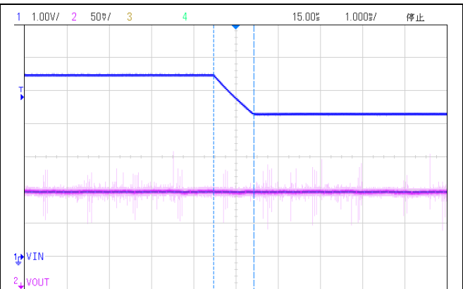
Input Transient Response
