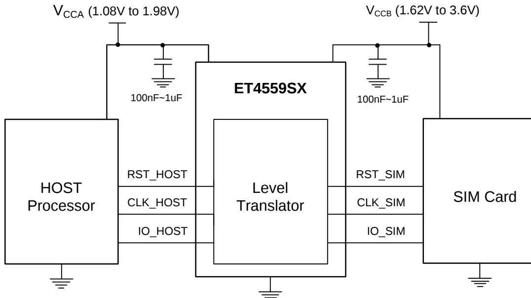
Figure 5. ET4559SX application circuit interfacing with typical SIM card
