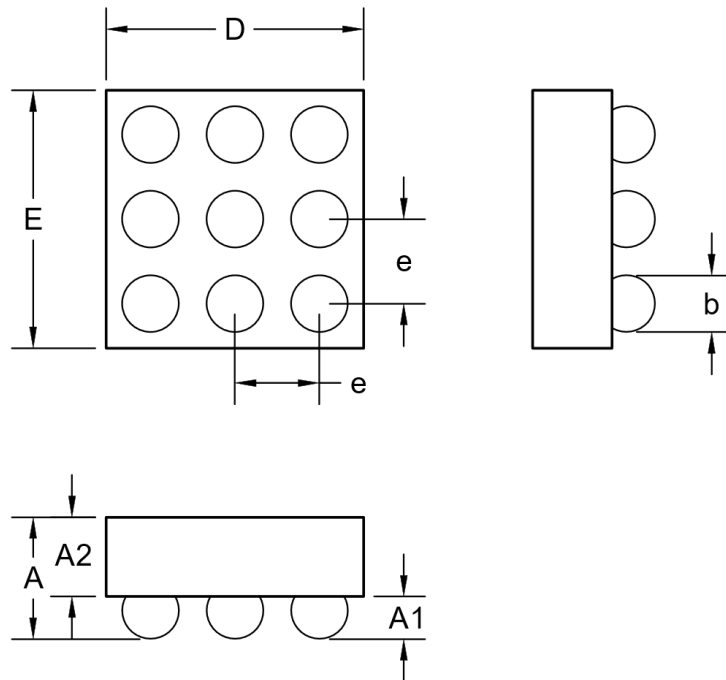
COMMON DIMENSIONS
