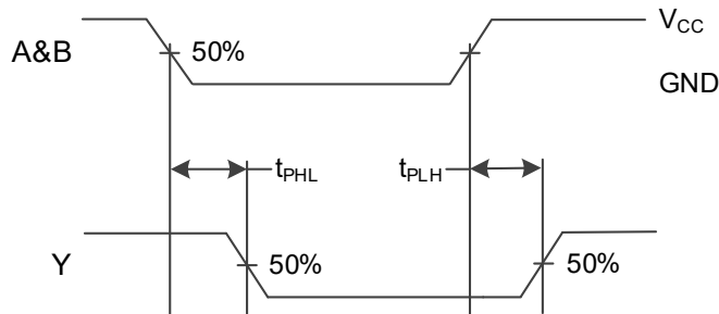
Figure 3. Switching Waveforms
