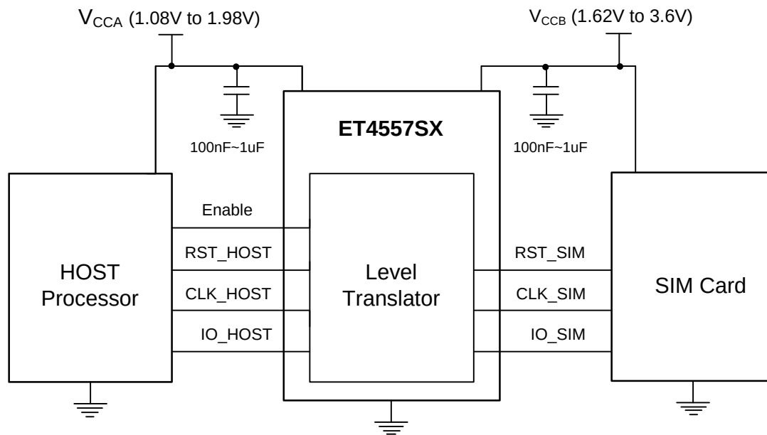
Figure 5. ET4557SX application circuit interfacing with typical SIM card
