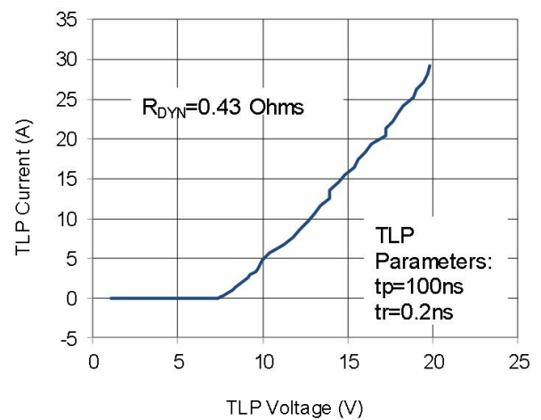
Figure 6: TLP Positive I-V Curve
