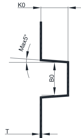
end view
