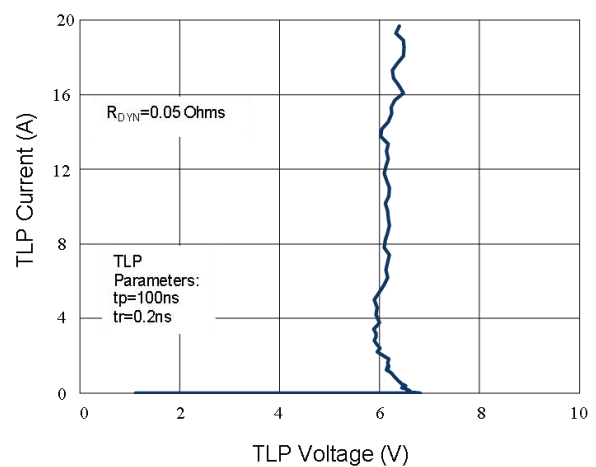
Figure 6: TLP Curve
