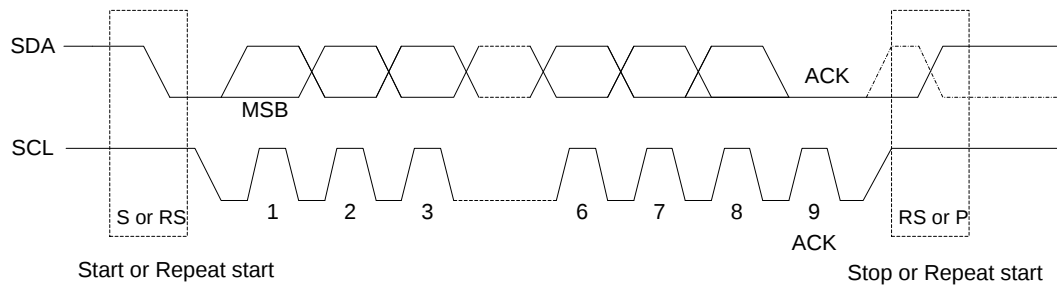
Figure1. I²C write mode
