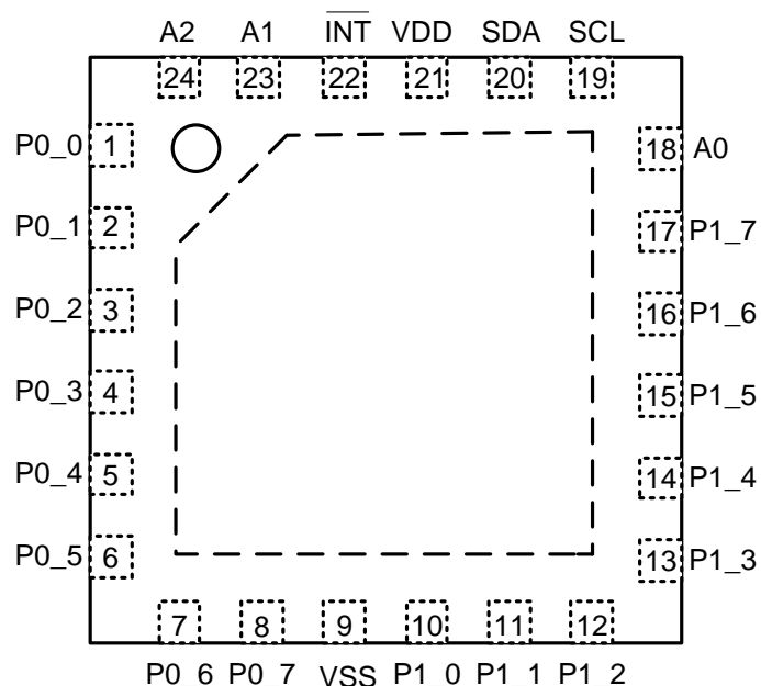
Figure 1. Pin Assignments (Top View)
