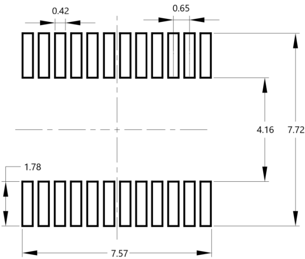
Land Pattern Recommendation Unit:mm
