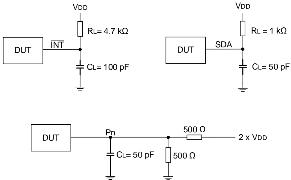
Figure 7. \overline{\text{INT}} 、SDA、Port P load configuration
