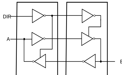
Fig 3. Logic symbol
