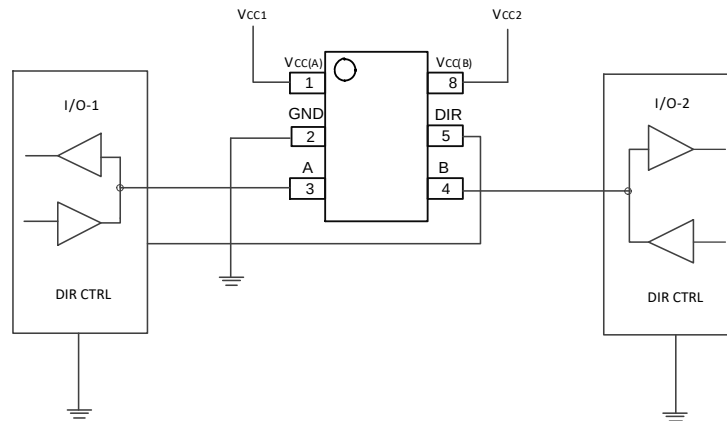
Fig.7 Application Circuits
