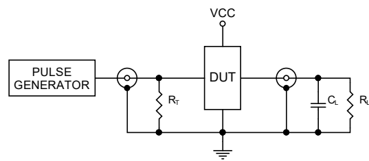
Figure 4. Test Circuit
