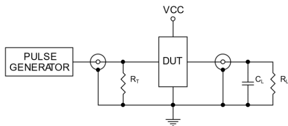
Figure4. Test Circuit
