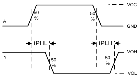
Figure 3. Switching Waveform
