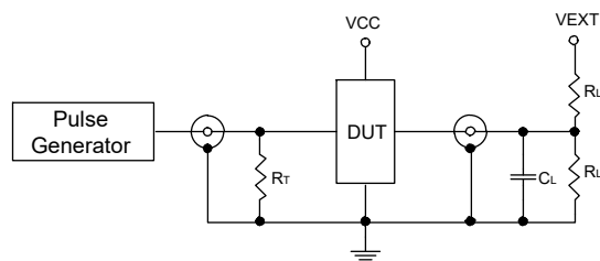
Figure4. Test Circuit
