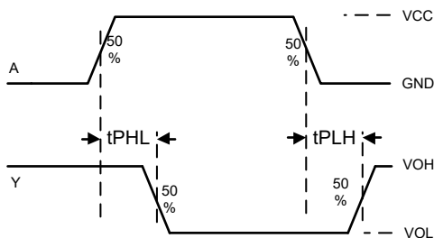
Figure 3. Switching Waveform
