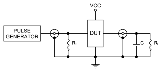
Figure 4. Test Circuit
