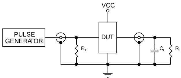
Figure4. Test Circuit
