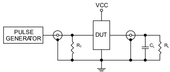
Figure4. Test Circuit
