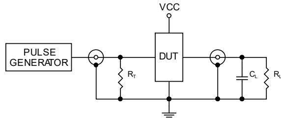
Figure4. Test Circuit
