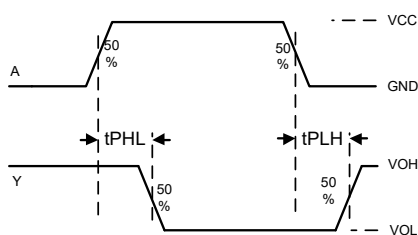
Figure 3. Switching Waveform
