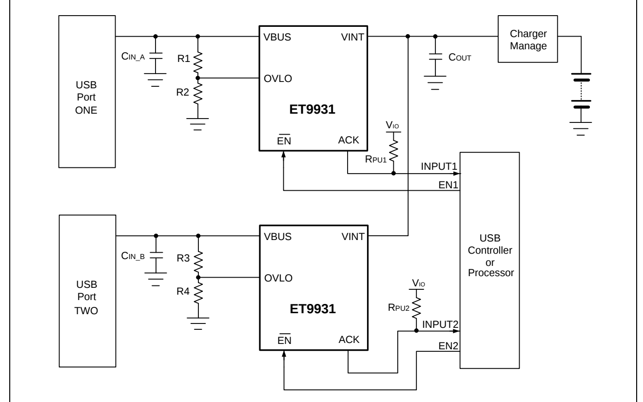
Figure 5. Application Circuit 2
