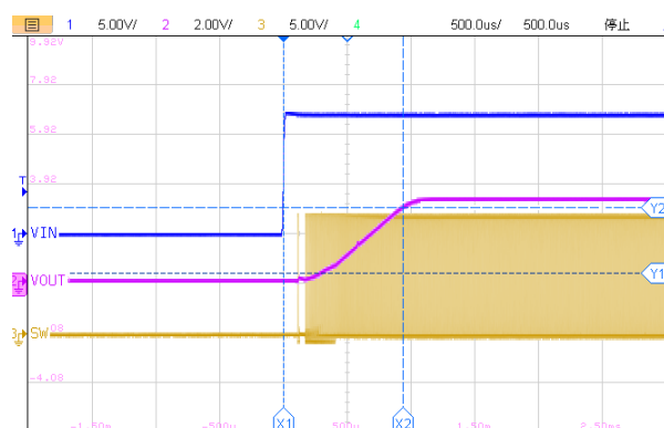
500us/div, V_{EN}=5V V_{OUT}=3.3V I_{OUT}=2A Figure36. ET81413 Start-Up Relative to V_{IN}
