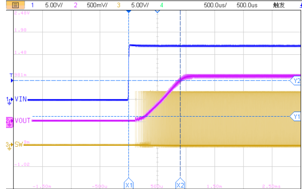
500us/div, V_{IN}=12V V_{OUT}=1V I_{OUT}=2A Figure34. ET81413 Start-Up Relative to V_{IN}
