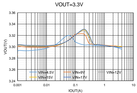
Figure10. ET81413 Load Regulation, V_{OUT}=3.3V
