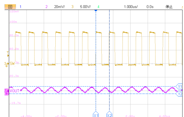
1us/div, V_{OUT}=5.0V I_{OUT}=4A Figure26. ET81413 Output Ripple
