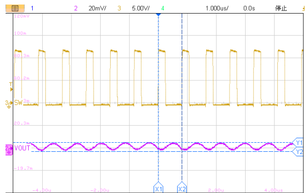
1us/div, V_{OUT}=3.3V I_{OUT}=4A Figure22. ET81413 Output Ripple
