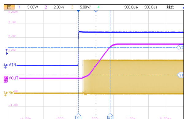
500us/div, V_{EN}=5V V_{OUT}=5.0V I_{OUT}=2A Figure38. ET81413 Start-Up Relative to V_{IN}
