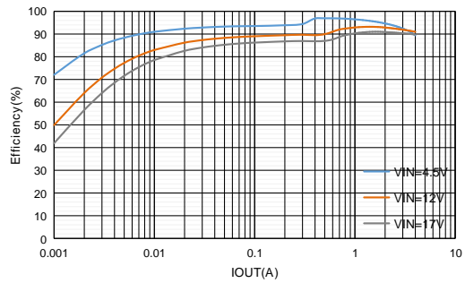
Figure7. ET81413 Efficiency vs Output Current
