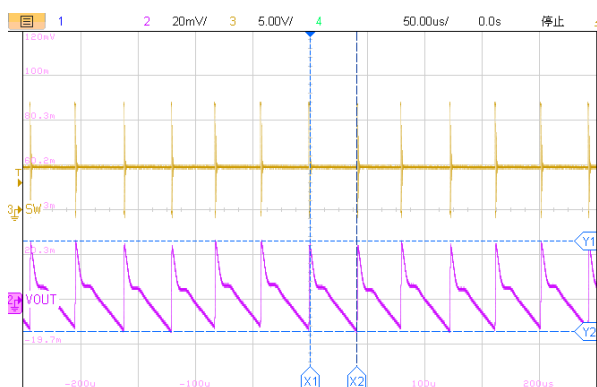
50us/div, V_{OUT}=5.0V I_{OUT}=10mA Figure23. ET81413 Output Ripple
