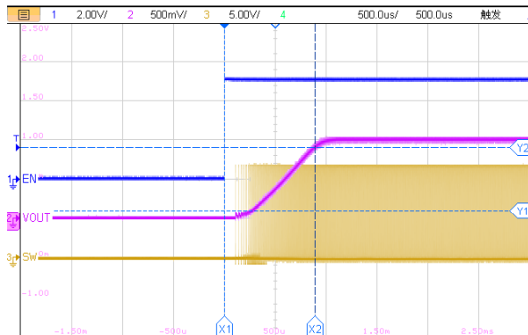
500us/div, V_{IN}=12V V_{OUT}=1.0V I_{OUT}=2A Figure33. ET81413 Start-Up Relative to EN
