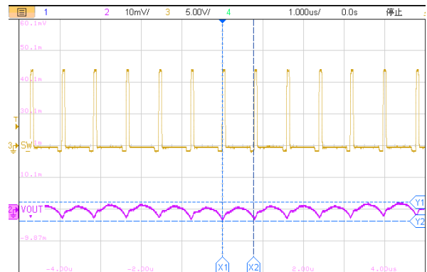
1us/div, V_{OUT}=1.0V I_{OUT}=500mA Figure16. ET81413 Output Ripple
