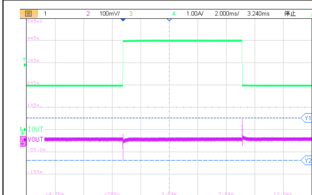
2ms/div, V_{OUT}=5.0V I_{OUT} = 2A to 4A Figure31. ET81413 Load Transient
