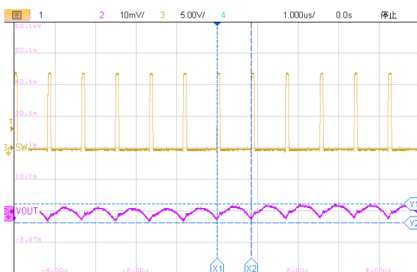
1us/div, V_{OUT}=1.0V I_{OUT}=2A Figure17. ET81413 Output Ripple
