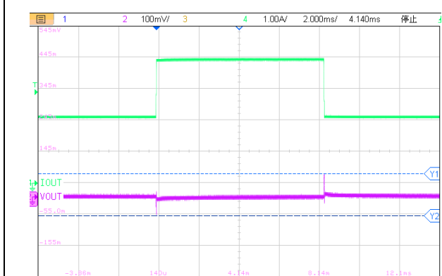
2ms/div, V_{OUT}=3.3V I_{OUT} = 2A to 4A Figure29. ET81413 Load Transient
