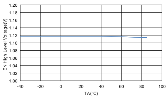
Figure3. ET81413 EN_H vs Temperature
