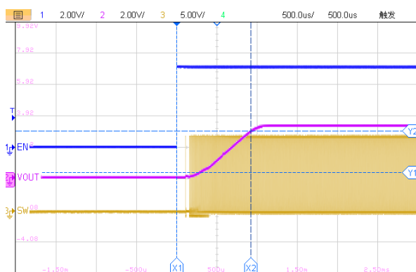
500us/div, V_{IN}=12V V_{OUT}=3.3V I_{OUT}=2A Figure35. ET81413 Start-Up Relative to EN
