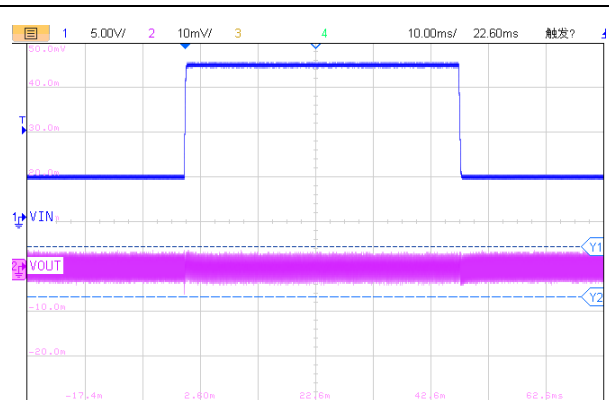
10ms/div, V_{OUT}=1V I_{OUT} = 2A V_{IN}=4.5V to 17V Figure28. ET81413 Line Transient
