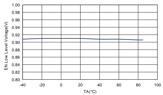
Figure4. ET81413 EN_L vs Temperature
