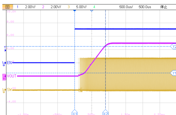
500us/div, V_{EN}=5V V_{OUT}=5.0V I_{OUT}=2A Figure37. ET81413 Start-Up Relative to EN
