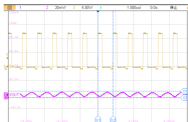
1us/div, V_{OUT}=3.3V I_{OUT}=500mA Figure20. ET81413 Output Ripple
