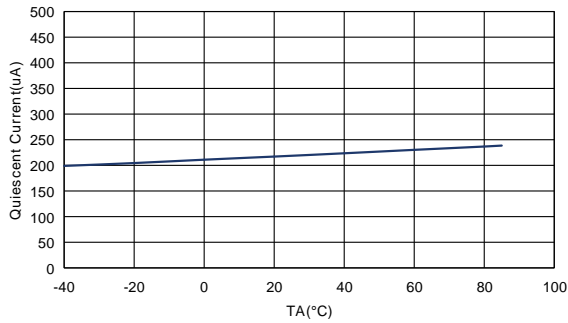
Figure1. ET81413 Quiescent current vs Temperature
