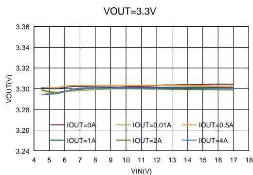
Figure13. ET81413 Line Regulation, V_{OUT}=3.3V
