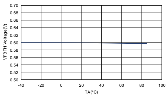
Figure5. ET81413 V_{FB} Voltage vs Temperature
