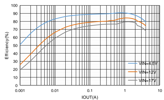
Figure6. ET81413 Efficiency vs Output Current
