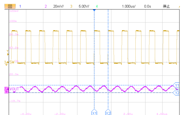
1us/div, V_{OUT}=5.0V I_{OUT}=500mA Figure24. ET81413 Output Ripple
