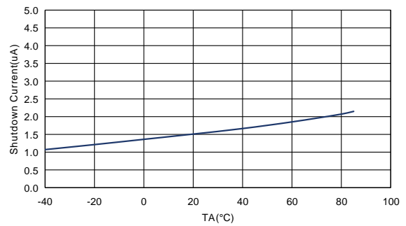
Figure2. ET81413 Shutdown current vs Temperature
