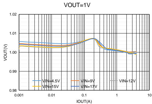
Figure9. ET81413 Load Regulation, V_{OUT}=1.0V
