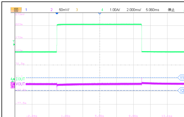
2ms/div, V_{OUT}=1.0V I_{OUT} = 2A to 4A Figure27. ET81413 Load Transient
