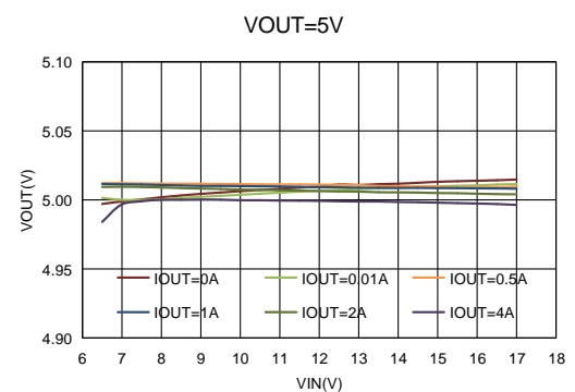
Figure14. ET81413 Line Regulation, V_{OUT}=5.0V
