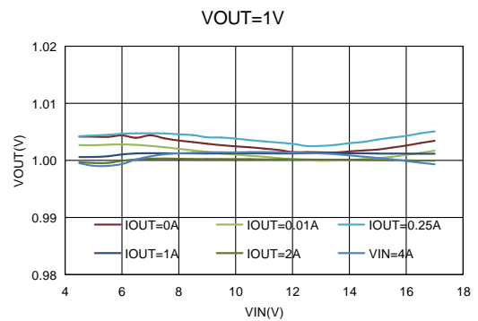
Figure12. ET81413 Line Regulation, V_{OUT}=1.0V
