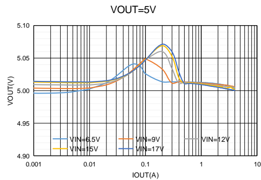
Figure11. ET81413 Load Regulation, V_{OUT}=5.0V
