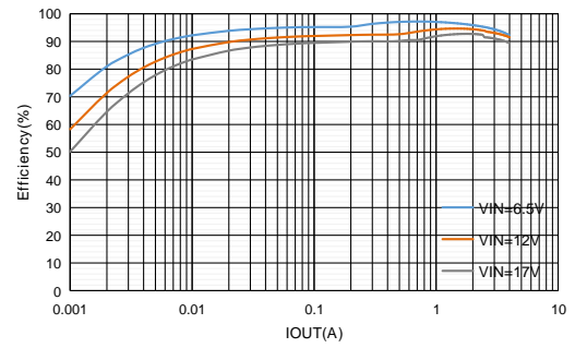
Figure8. ET81413 Efficiency vs Output Current
