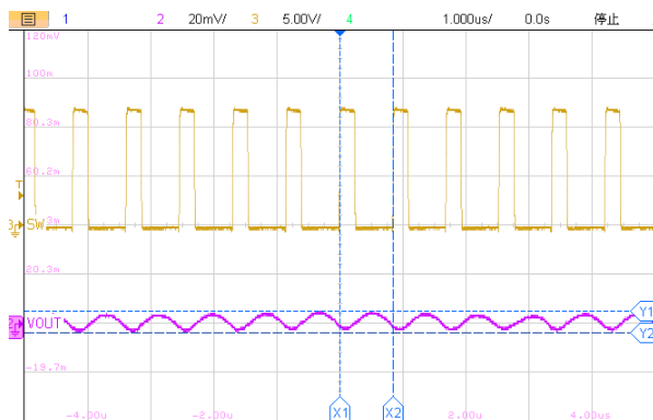
1us/div, V_{OUT}=3.3V I_{OUT}=2A Figure21. ET81413 Output Ripple
