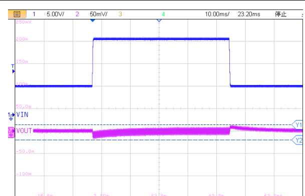
10ms/div, V_{OUT}=5V I_{OUT} = 2A V_{IN}=6.5V to 17V Figure32. ET81413 Line Transient
