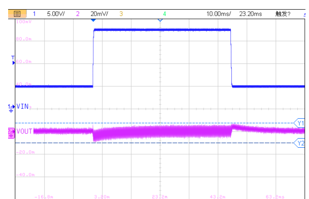
10ms/div, V_{OUT}=3.3V I_{OUT} = 2A V_{IN}=4.5V to 17V Figure30. ET81413 Line Transient
