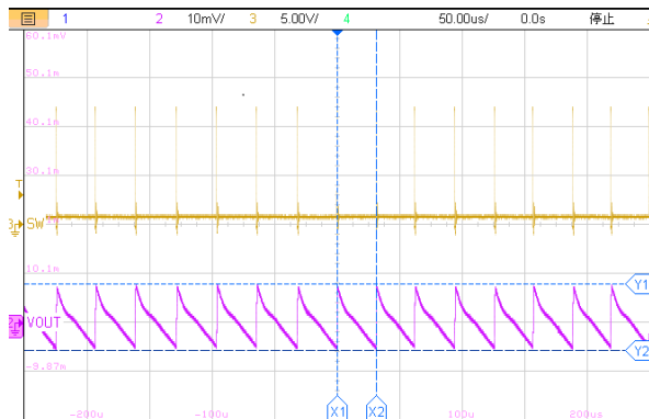
50us/div, V_{OUT}=1.0V I_{OUT}=10mA Figure15. ET81413 Output Ripple
