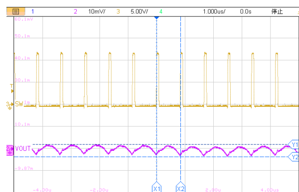
1us/div, V_{OUT}=1V I_{OUT}=4A Figure18. ET81413 Output Ripple
