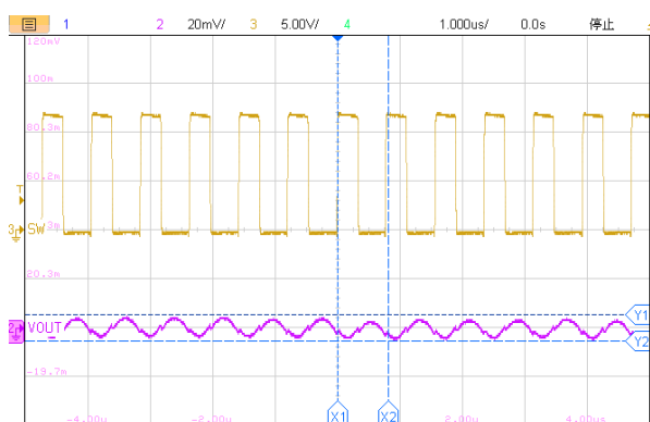
1us/div, V_{OUT}=5.0V I_{OUT}=2A Figure25. ET81413 Output Ripple
