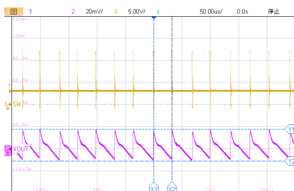
50us/div, V_{OUT}=3.3V I_{OUT}=10mA Figure19. ET81413 Output Ripple
