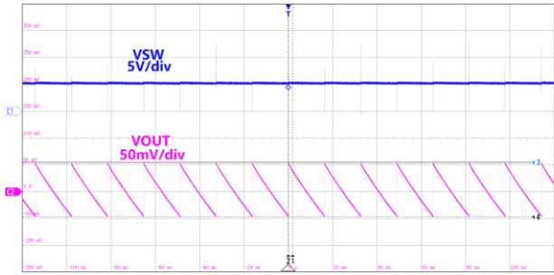
Figure19.Switch&Ripple Waveform VIN=12V,VOUT=5.0V,IOUT=0A
