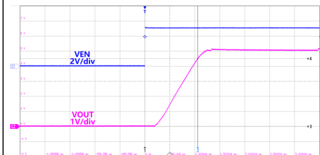
Figure39.Soft Start
