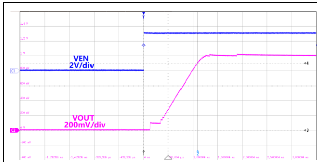
Figure35.Soft Start
