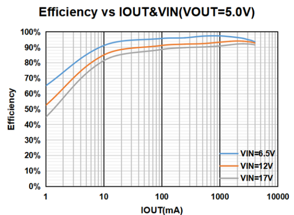
Figure10.Efficiency vs IOUT&VIN,VOUT=5.0V
