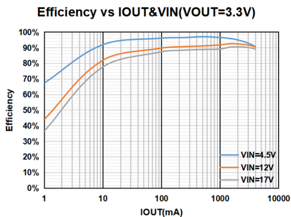
Figure9.Efficiency vs IOUT&VIN,VOUT=3.3V
