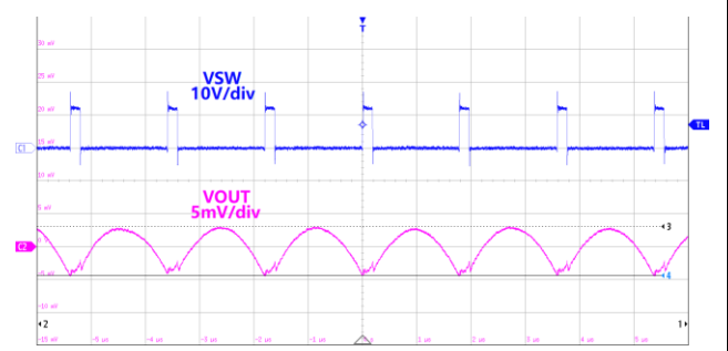
Figure14.Switch&Ripple Waveform V_{IN}=12V, V_{OUT}=1.0V, I_{OUT}=4A
