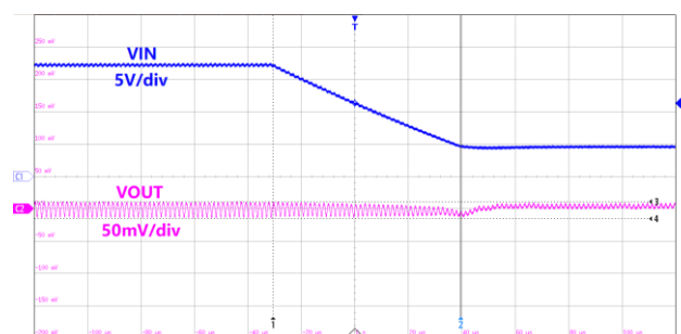
Figure32.Line Transient VIN=17~4.5V,VOUT=3.3V,IOUT=2A
