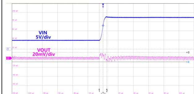
Figure29.Line Transient VIN=4.5~17V,VOUT=1.0V,IOUT=2A
