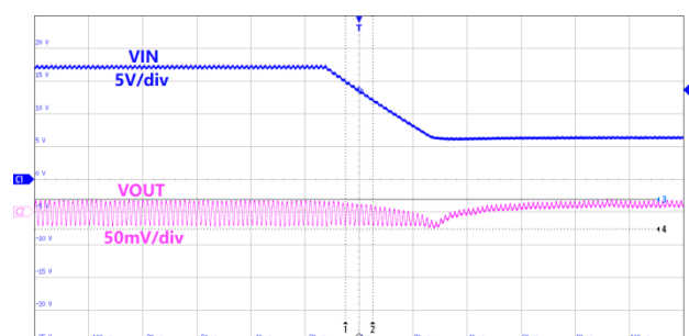
Figure34.Line Transient VIN=17~6.5V,VOUT=5.0V,IOUT=2A
