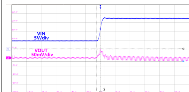
Figure31.Line Transient VIN=4.5~17V,VOUT=3.3V,IOUT=2A
