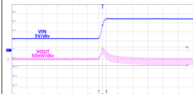
Figure33.Line Transient VIN=6.5~17V,VOUT=5.0V,IOUT=2A
