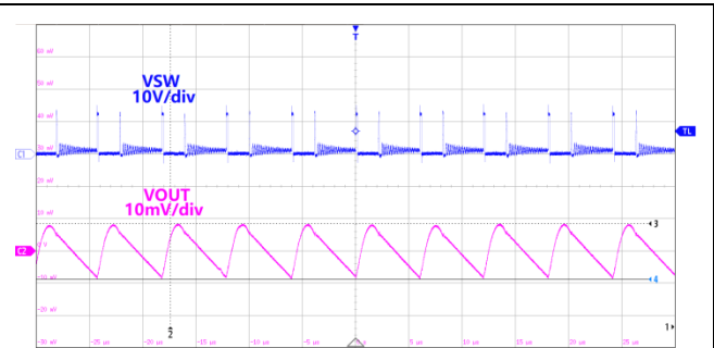
Figure12.Switch&Ripple Waveform V_{IN}=12V, V_{OUT}=1.0V, I_{OUT}=0.1A
