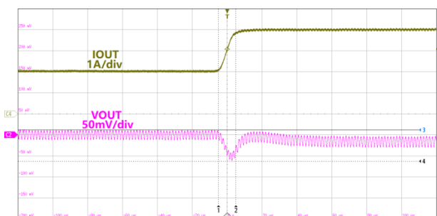
Figure25.Load Transient VIN=12V,VOUT=3.3V,IOUT=2~4A
