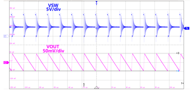
Figure20.Switch&Ripple Waveform VIN=12V,VOUT=5.0V,IOUT=0.1A
