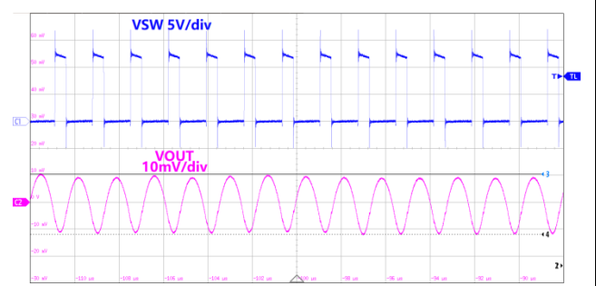
Figure18.Switch&Ripple Waveform V_{IN}=12V, V_{OUT}=3.3V, I_{OUT}=4A
