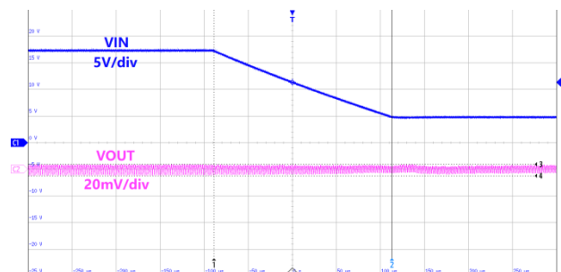
Figure30.Line Transient VIN=17~4.5V,VOUT=1.0V,IOUT=2A
