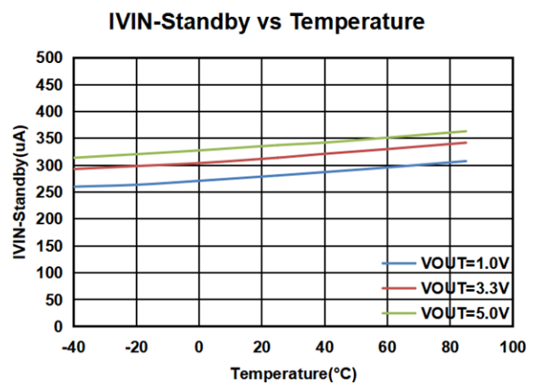
Figure2.IVIN-Standby vs Temperature
