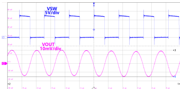
Figure21.Switch&Ripple Waveform VIN=12V,VOUT=5.0V,IOUT=2A
