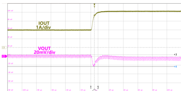
Figure23.Load Transient VIN=12V,VOUT=1.0V,IOUT=2~4A
