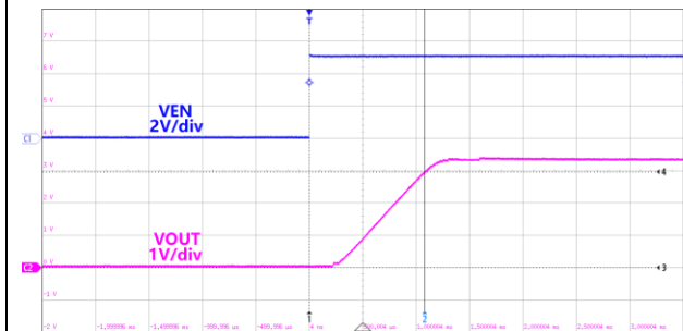
Figure37.Soft Start
