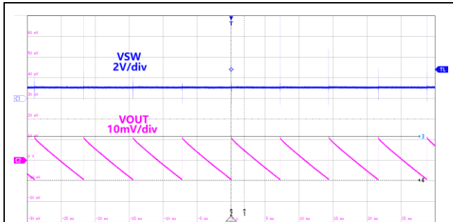
Figure11.Switch&Ripple Waveform V_{IN}=12V, V_{OUT}=1.0V, I_{OUT}=0A
