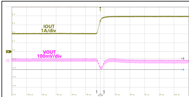
Figure27.Load Transient VIN=12V,VOUT=5.0V,IOUT=2~4A
