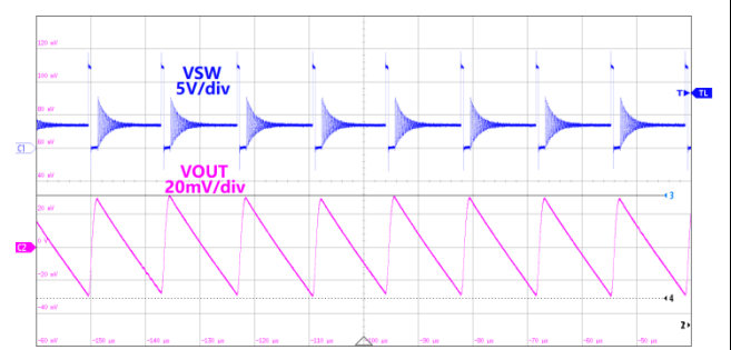
Figure16.Switch&Ripple Waveform V_{IN}=12V, V_{OUT}=3.3V, I_{OUT}=0.1A
