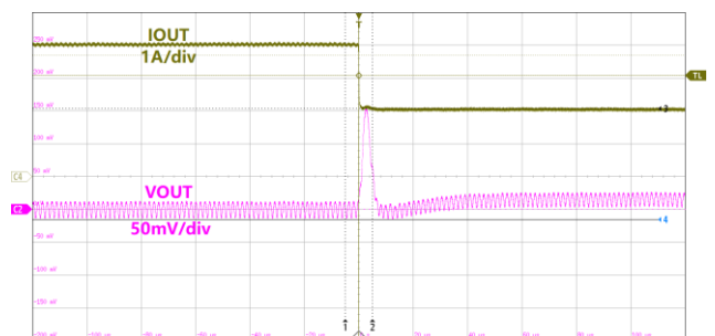
Figure26.Load Transient VIN=12V,VOUT=3.3V,IOUT=4~2A
