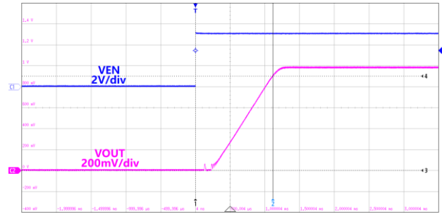
Figure36.Soft Start
