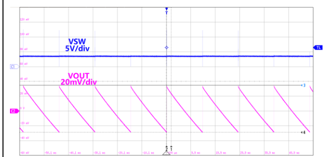
Figure15.Switch&Ripple Waveform V_{IN}=12V, V_{OUT}=3.3V, I_{OUT}=0A
