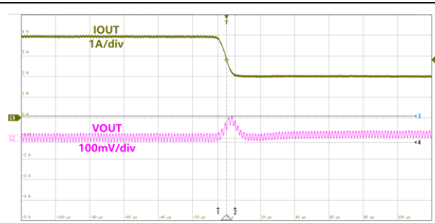
Figure28.Load Transient VIN=12V,VOUT=5.0V,IOUT=4~2A
