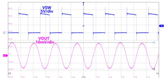
Figure22.Switch&Ripple Waveform VIN=12V,VOUT=5.0V,IOUT=4A
