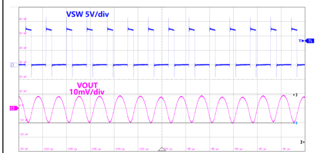
Figure17.Switch&Ripple Waveform V_{IN}=12V, V_{OUT}=3.3V, I_{OUT}=2A
