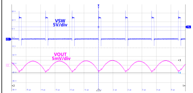
Figure13.Switch&Ripple Waveform V_{IN}=12V, V_{OUT}=1.0V, I_{OUT}=2A
