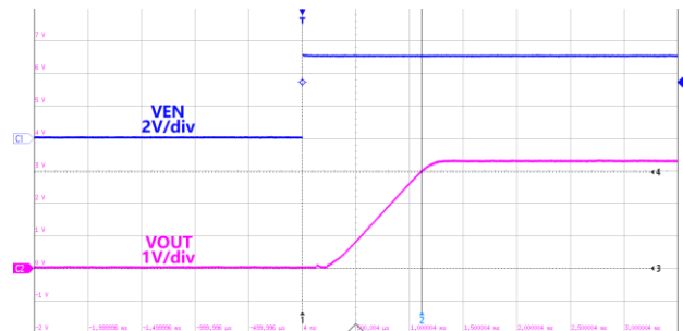
Figure38.Soft Start
