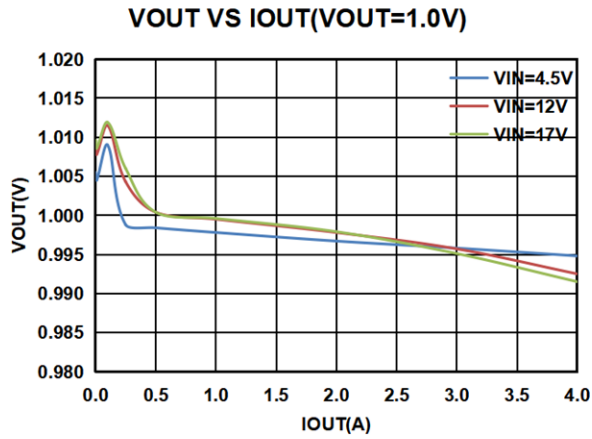
Figure5.VOUT vs IOUT,VOUT=1.0V
