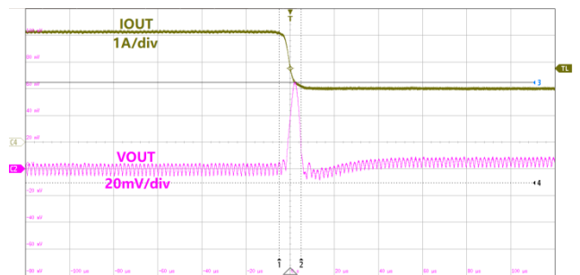
Figure24.Load Transient VIN=12V,VOUT=1.0V,IOUT=4~2A
