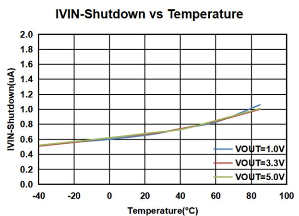
Figure4.IVIN-Shutdown vs Temperature
