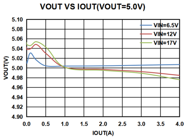
Figure7.VOUT vs IOUT,VOUT=5.0V
