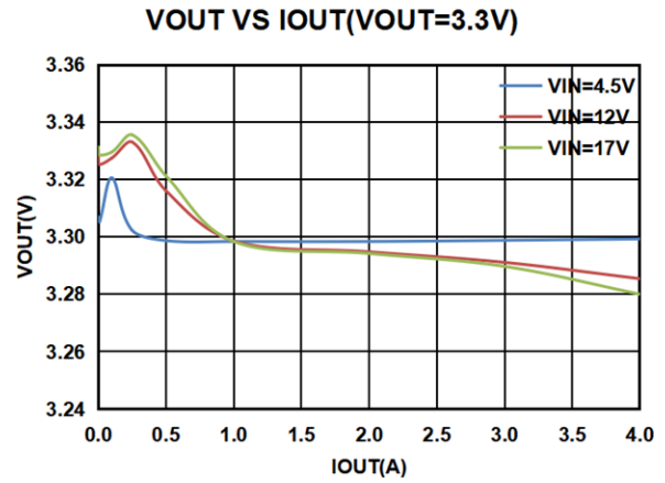
Figure6.VOUT vs IOUT,VOUT=3.3V
