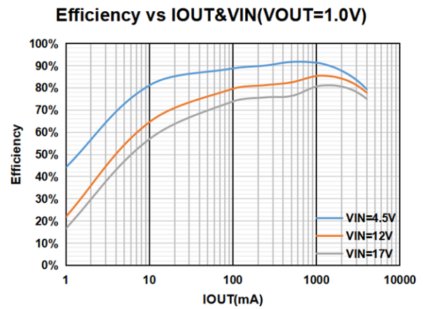
Figure8.Efficiency vs IOUT&VIN,VOUT=1.0V
