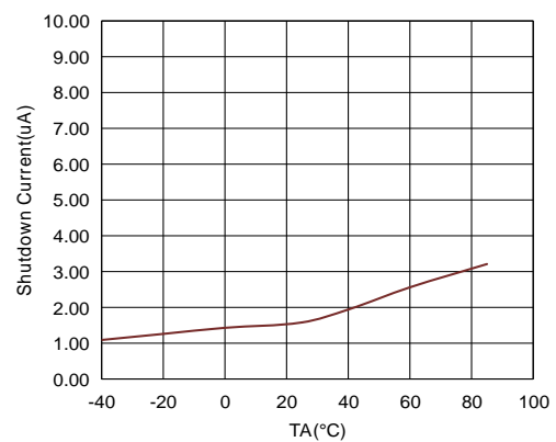
Figure2. ET81313 Shutdown current vs Temperature
