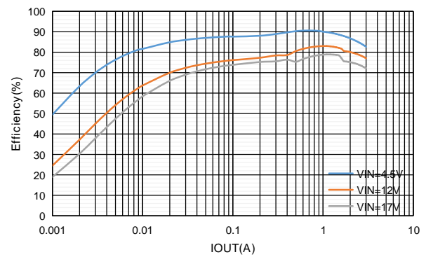
Figure6. ET81313 Efficiency vs Output Current
