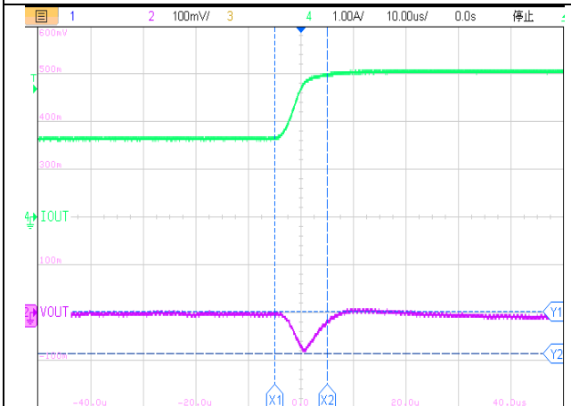
10us/div, V_{OUT}=3.3V I_{OUT} = 1.5A to 3A Figure29. ET81313 Load Transient
