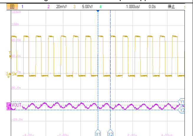
1us/div, V_{OUT}=5.0V I_{OUT}=3A Figure26. ET81313 Output Ripple
