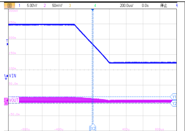
Figure34. ET81313 Line Transient
