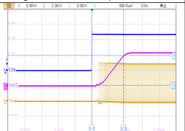
Figure42. ET81313 Start-Up Relative to V_{IN}
