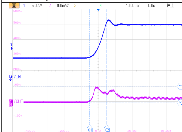
Figure35. ET81313 Line Transient
