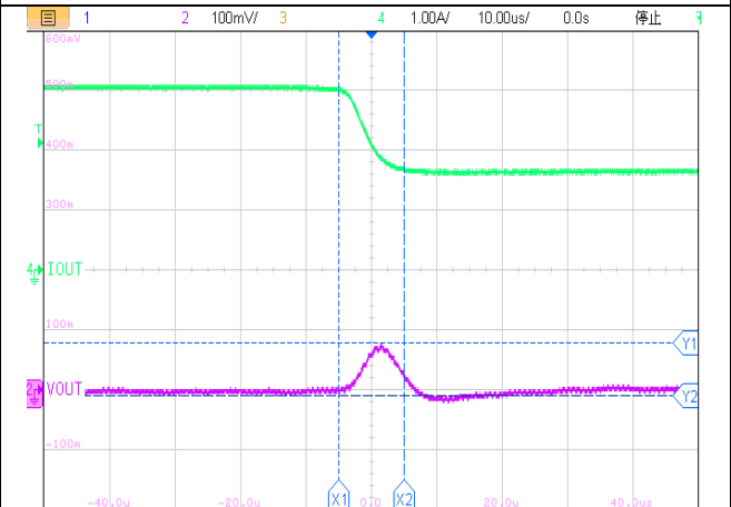
10us/div, V_{OUT}=3.3V I_{OUT} = 3A to 1.5A Figure30. ET81313 Load Transient
