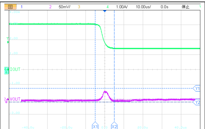
10us/div, V_{OUT}=1.0V I_{OUT} = 3A to 1.5A Figure28. ET81313 Load Transient
