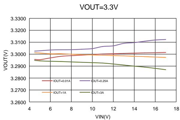
Figure13. ET81313 Line Regulation, V_{OUT}=3.3V
