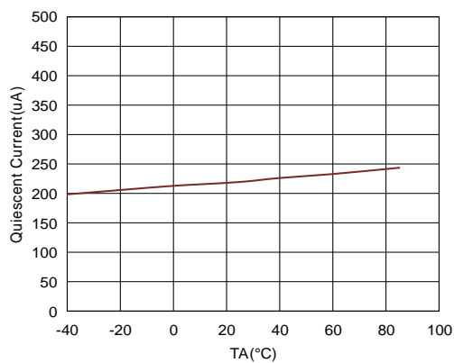
Figure1. ET81313 Quiescent current vs Temperature
