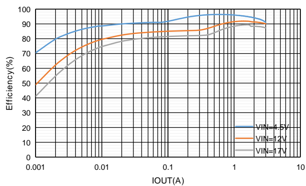
Figure7. ET81313 Efficiency vs Output Current
