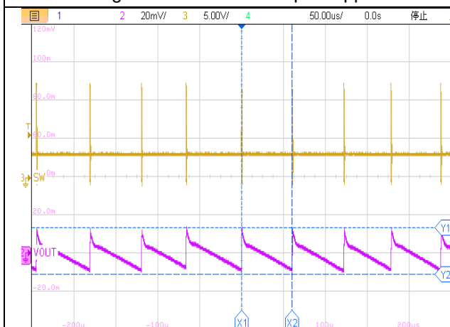
Figure17. ET81313 Output Ripple
