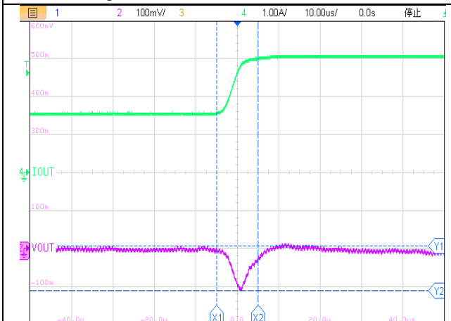
10us/div, V_{OUT}=5.0V I_{OUT} = 1.5A to 3A Figure31. ET81313 Load Transient
