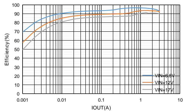
Figure8. ET81313 Efficiency vs Output Current
