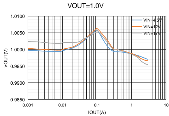
Figure9. ET81313 Load Regulation, V_{OUT}=1.0V
