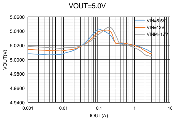
Figure11. ET81313 Load Regulation, V_{OUT}=5.0V
