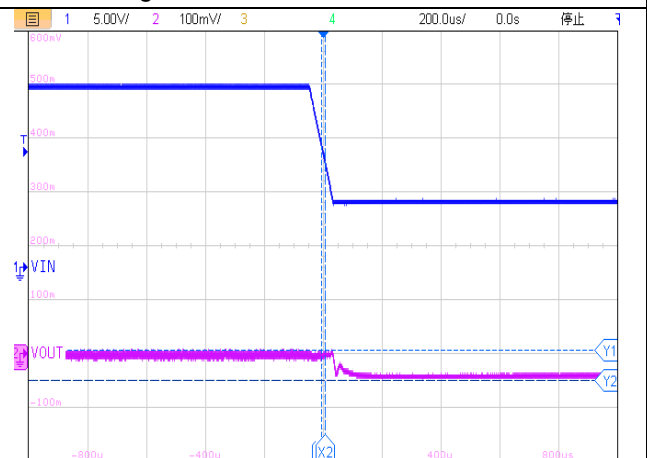
Figure36. ET81313 Line Transient
