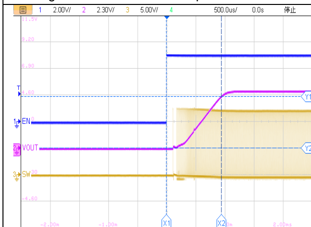
Figure41. ET81313 Start-Up Relative to EN
