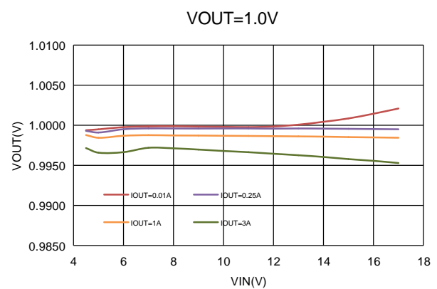
Figure12. ET81313 Line Regulation, V_{OUT}=1.0V
