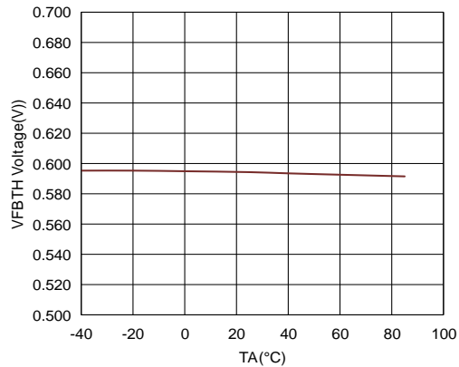
Figure5. ET81313 V_{FB} Voltage vs Temperature
