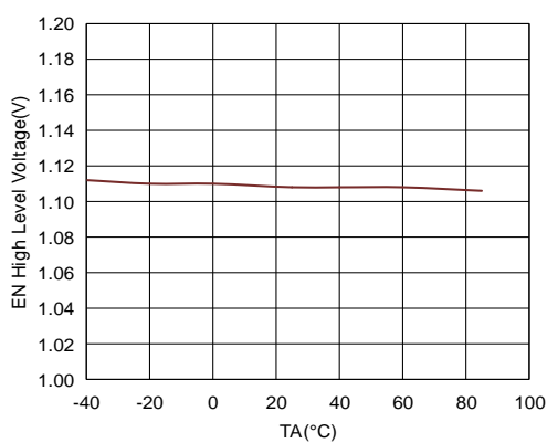
Figure3. ET81313 EN_H vs Temperature
