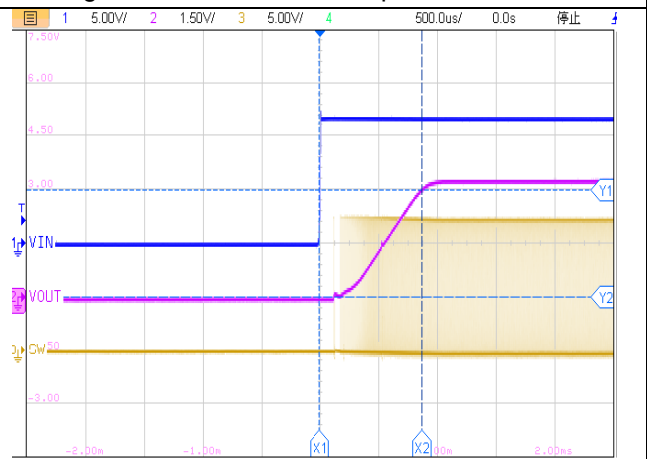
Figure40. ET81313 Start-Up Relative to V_{IN}
