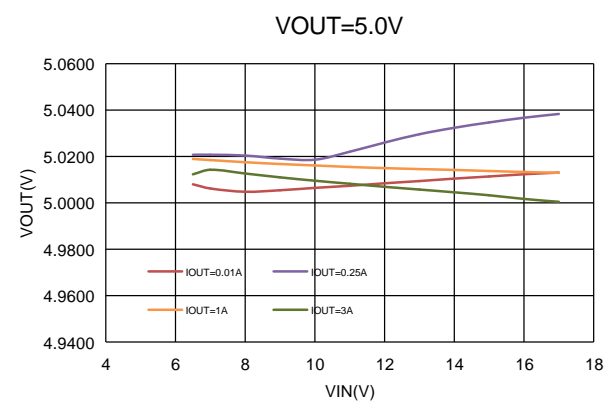
Figure14. ET81313 Line Regulation, V_{OUT}=5.0V
