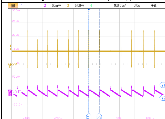
100us/div, V_{OUT}=5.0V I_{OUT}=10mA Figure23. ET81313 Output Ripple
