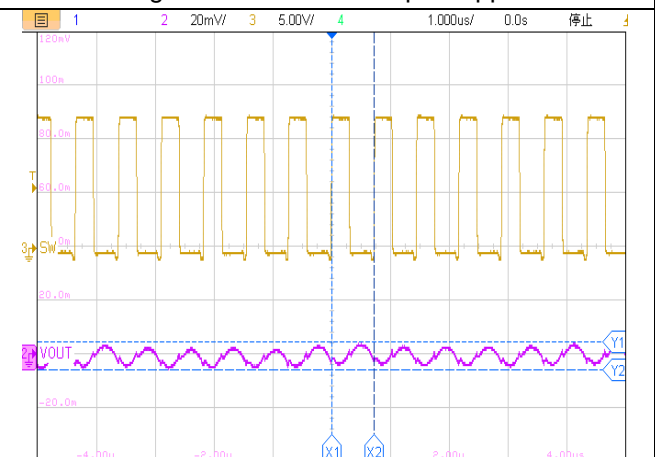
1us/div, V_{OUT}=5.0V I_{OUT}=500mA Figure24. ET81313 Output Ripple
