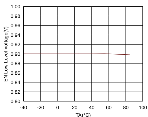
Figure4. ET81313 EN_L vs Temperature
