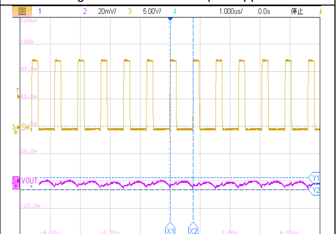
Figure18. ET81313 Output Ripple
