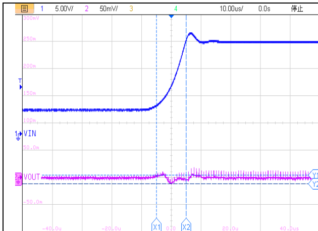
Figure33. ET81313 Line Transient
