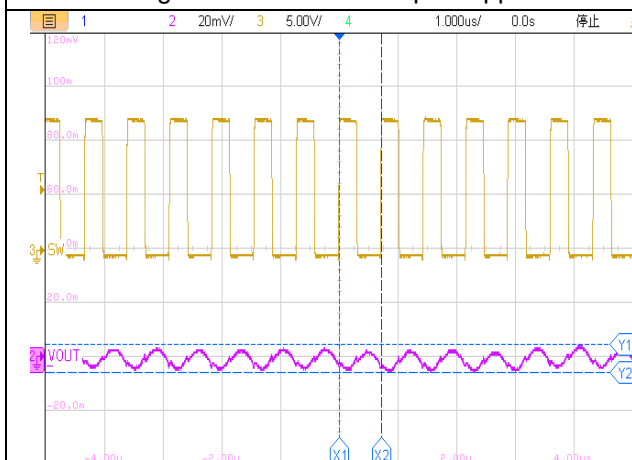
1us/div, V_{OUT}=5.0V I_{OUT}=1.5A Figure25. ET81313 Output Ripple
