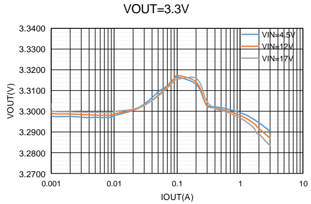
Figure10. ET81313 Load Regulation, V_{OUT}=3.3V
