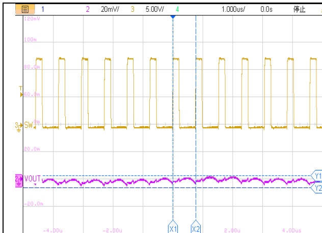
1us/div, V_{OUT}=3.3V I_{OUT}=1.5A Figure21. ET81313 Output Ripple
