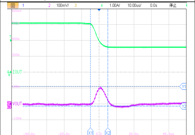
10us/div, V_{OUT}=5.0V I_{OUT} = 3A to 1.5A Figure32. ET81313 Load Transient
