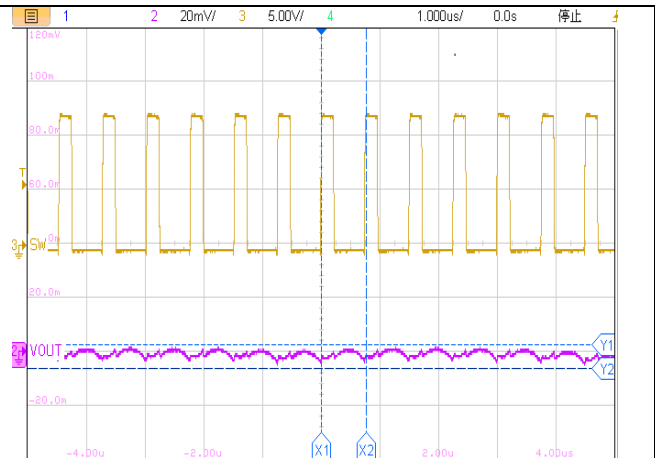
1us/div, V_{OUT}=3.3V I_{OUT}=3A Figure22. ET81313 Output Ripple
