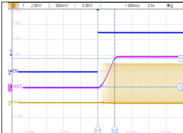
Figure39. ET81313 Start-Up Relative to EN
