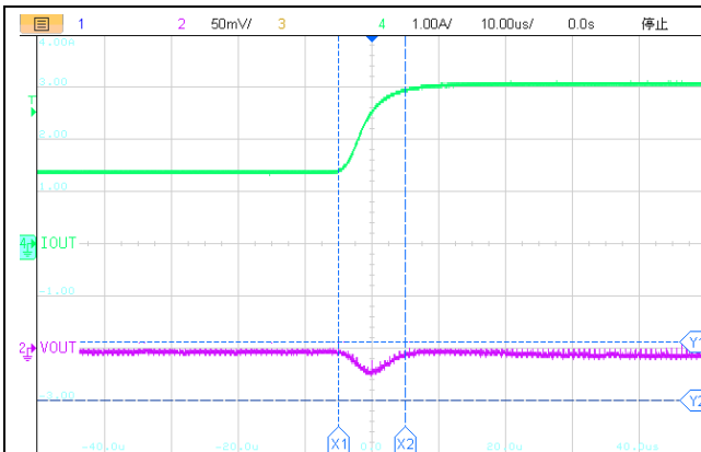
10us/div, V_{OUT}=1.0V I_{OUT} = 1.5A to 3A Figure27. ET81313 Load Transient
