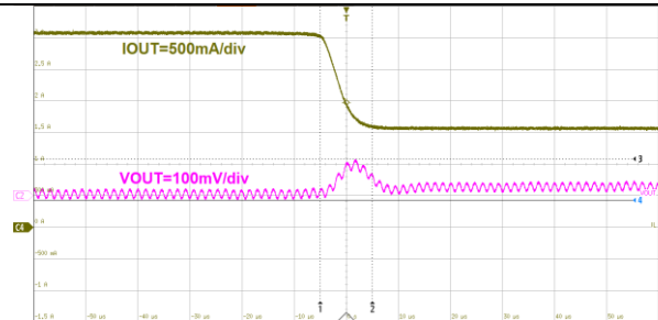
10us/div, V_{OUT}=5.0V I_{OUT} = 3A to 1.5A Figure34. ET81311 Load Transient
