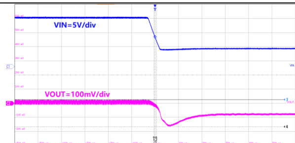
200us/div, V_{OUT}=5.0V I_{OUT} = 1.5A V_{IN}=17V to 6.5V Figure40. ET81311 Line Transient
