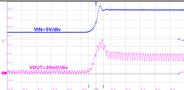
10us/div, V_{OUT}=3.3V I_{OUT} = 1.5A V_{IN}=4.5V to 17V Figure37. ET81311 Line Transient
