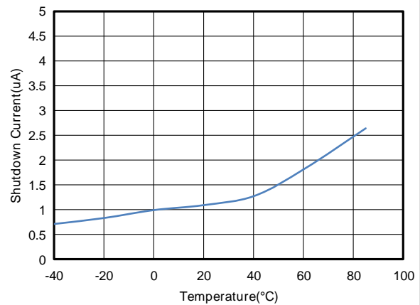
Figure2. ET81311 Shutdown current vs Temperature
