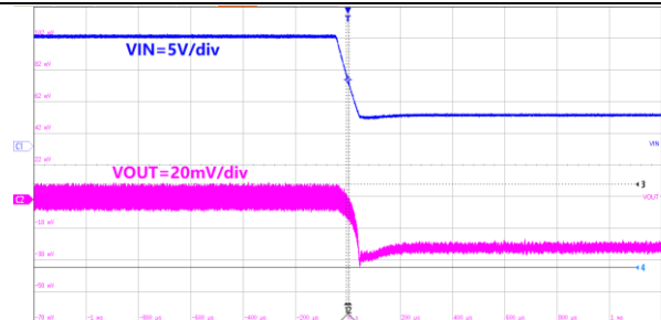
200us/div, V_{OUT}=3.3V I_{OUT} = 1.5A V_{IN}=17V to 4.5V Figure38. ET81311 Line Transient
