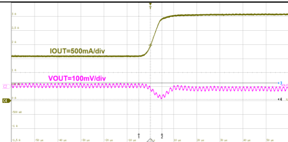
10us/div, V_{OUT}=5.0V I_{OUT} = 1.5A to 3A Figure33. ET81311 Load Transient
