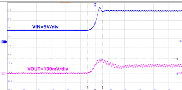
10us/div, V_{OUT}=5.0V I_{OUT} = 1.5A V_{IN}=6.5V to 17V Figure39. ET81311 Line Transient
