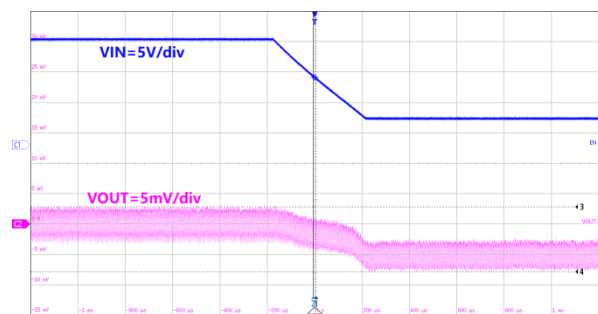
200us/div, V_{OUT}=1.0V I_{OUT} = 1.5A V_{IN}=17V to 4.5V Figure36. ET81311 Line Transient
