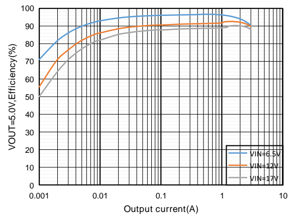
Figure8. ET81311 Efficiency vs Output Current
