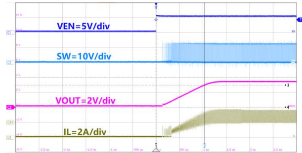
Figure42. ET81311 Start-Up Relative to EN
