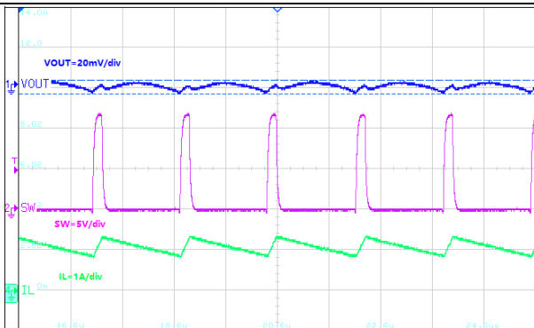
Figure23. ET8131AM V_{OUT}=1.05V Ripple(10mA)
