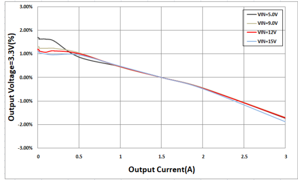
Figure13. ET8131AM Load Regulation, V_{OUT}=3.3V
