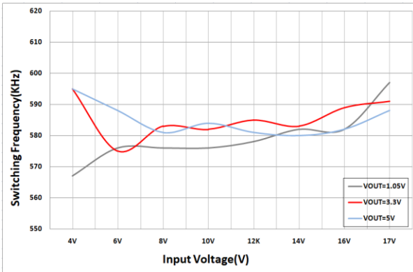
Figure5. Switching Frequency vs input Voltage
