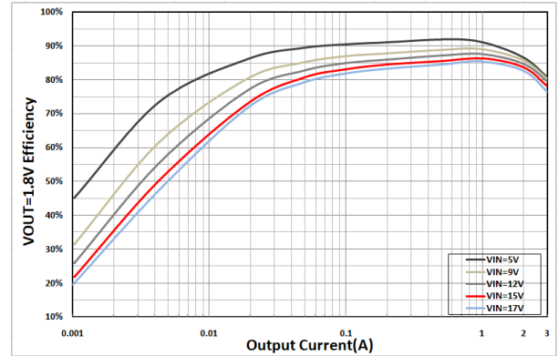
Figure8. V_{OUT}=1.8V Efficiency
