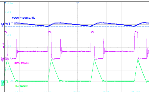
Figure25. ET8131AM V_{OUT}=1.05V Ripple (2A)
