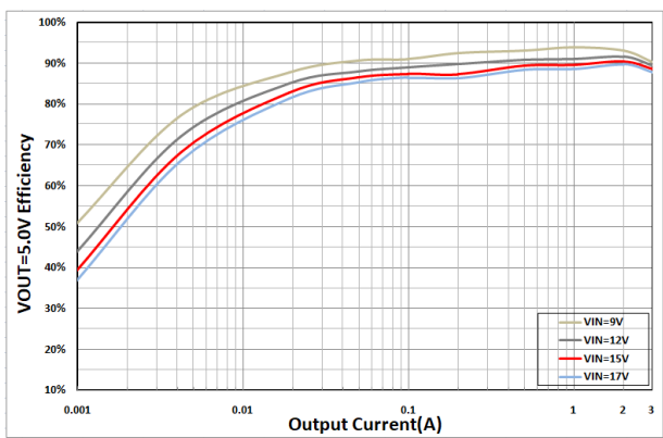
Figure11. V OUT =5.0V Efficiency L=2.2uH
