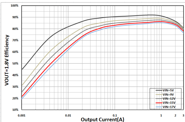
Figure9. V_{OUT}=1.8V Efficiency
