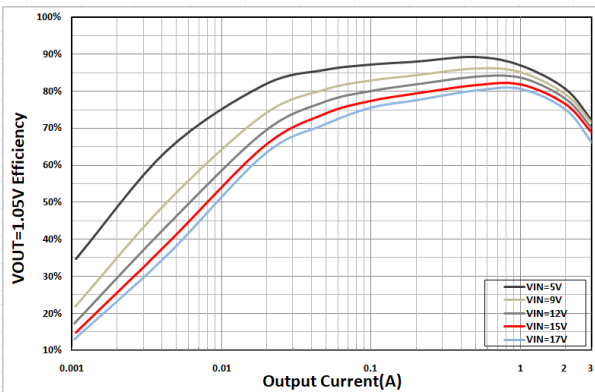
Figure7. V_{OUT}=1.05V Efficiency
