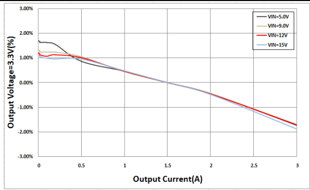
Figure13. ET8131 Load Regulation, V_{OUT}=3.3V
