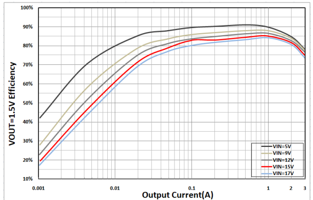
Figure8. V_{OUT}=1.5V Efficiency
