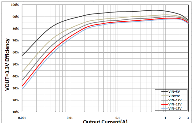
Figure10. V_{OUT}=3.3V Efficiency
