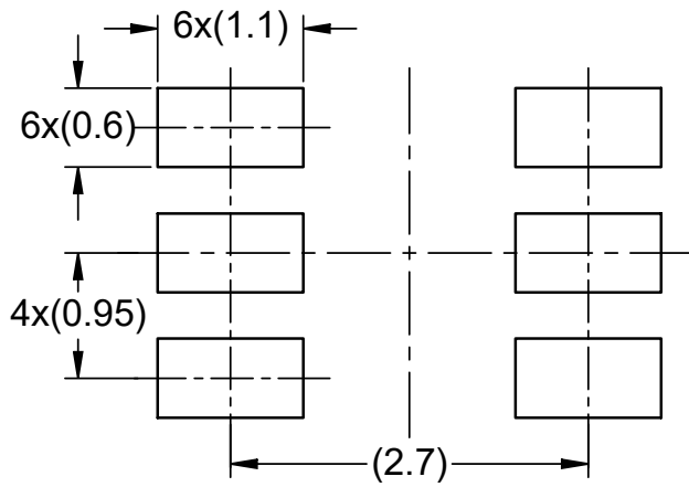
LAND PATTERN EXAMPLE
