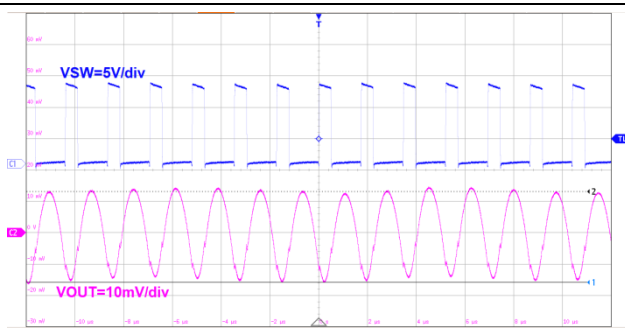
2us/div V_{OUT}=3.3V I_{OUT}=2A Figure22. ET8121 Output Ripple
