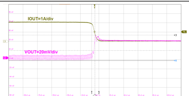
20us/div V_{OUT}=1.0V I_{OUT}=2A to 0A Figure27. ET8121 Load Transient
