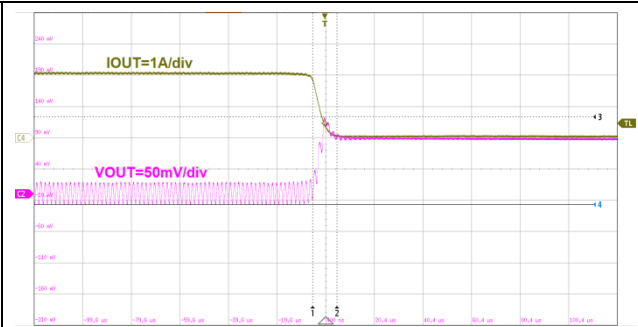
20us/div V_{OUT}=3.3V I_{OUT}=2A to 0A Figure31. ET8121 Load Transient
