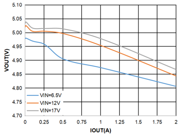
Figure10. ET8121 Load Regulation, V_{OUT}=5.0V
