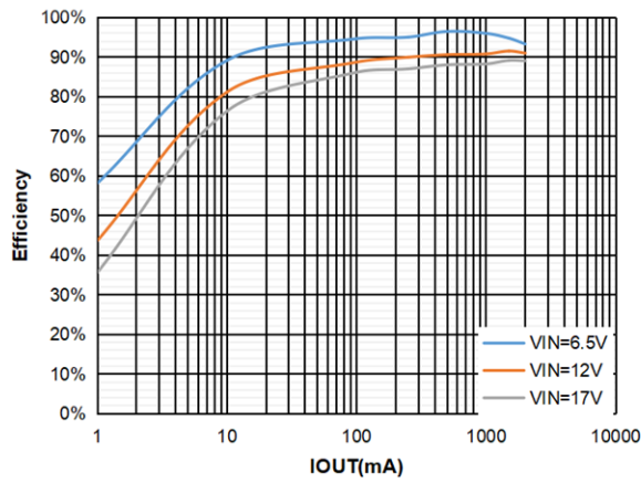
Figure7. V_{OUT}=5.0V Efficiency, L=2.2\mu H
