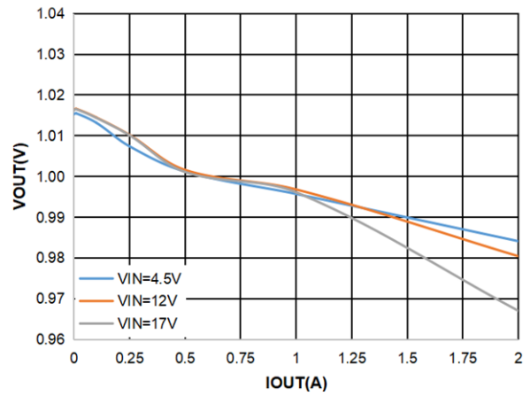
Figure8. ET8121 Load Regulation, V_{OUT}=1.0V
