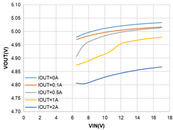
Figure13. ET8121 Line Regulation, V_{OUT}=5.0V
