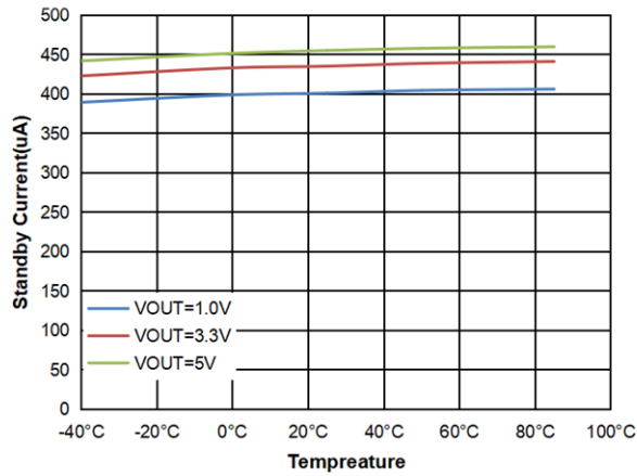
Figure1. ET8121 Standby Current vs Temperature
