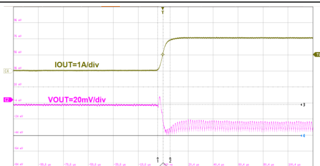
20us/div V_{OUT}=1.0V I_{OUT}=0A to 2A Figure26. ET8121 Load Transient
