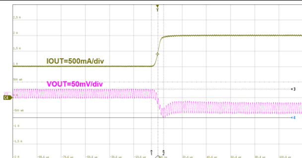
20us/div V_{OUT}=3.3V I_{OUT}=1A to 2A Figure32. ET8121 Load Transient
