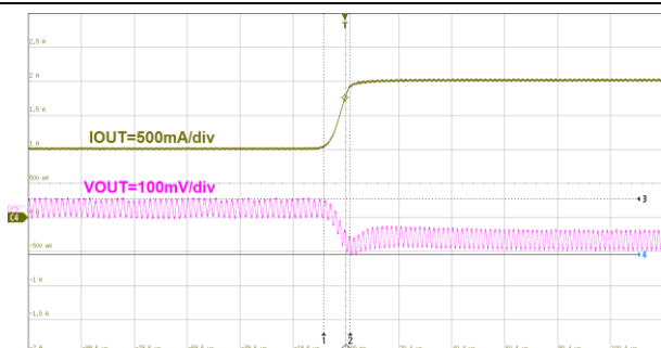
20us/div V_{OUT}=5V I_{OUT}=1A to 2A Figure36. ET8121 Load Transient
