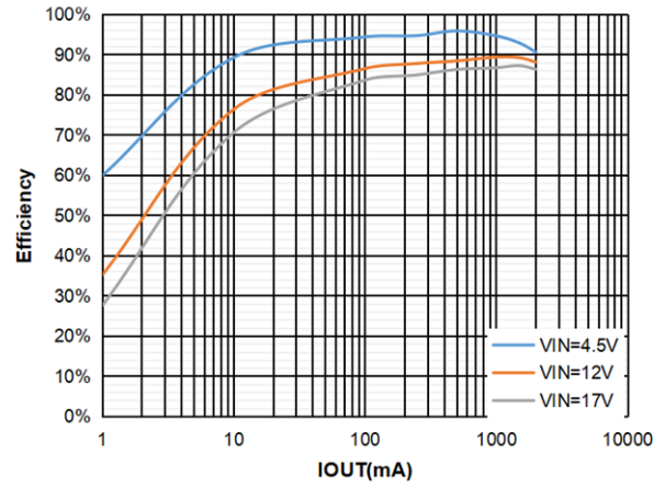
Figure6. V_{OUT}=3.3V Efficiency, L=2.2\mu H
