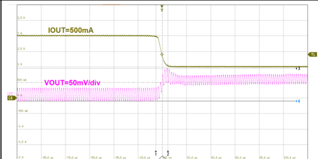
20us/div V_{OUT}=3.3V I_{OUT}=2A to 1A Figure33. ET8121 Load Transient
