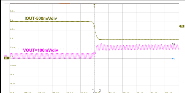
20us/div V_{OUT}=5V I_{OUT}=2A to 1A Figure37. ET8121 Load Transient
