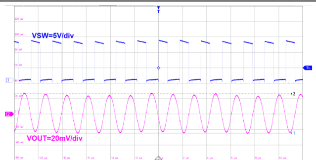
2us/div V_{OUT}=5.0V I_{OUT}=2A Figure25. ET8121 Output Ripple
