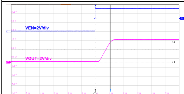
Figure14. ET8121 Start-Up Relative to EN
