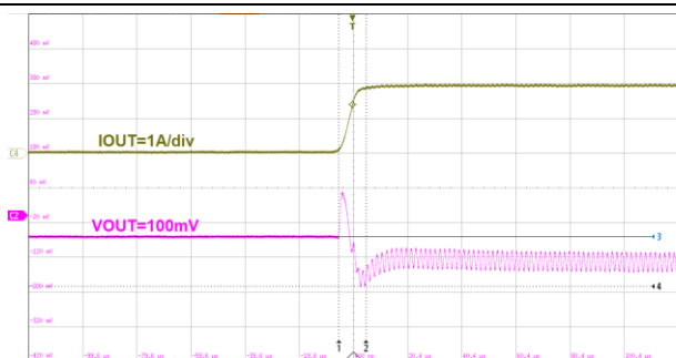
20us/div V_{OUT}=5V I_{OUT}=0A to 2A Figure34. ET8121 Load Transient
