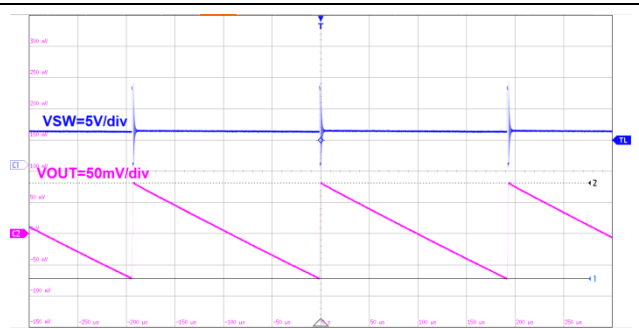
50us/div V_{OUT}=5.0V I_{OUT}=0.01A Figure23. ET8121 Output Ripple
