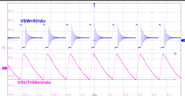
5us/div V_{OUT}=5.0V I_{OUT}=0.25A Figure24. ET8121 Output Ripple
