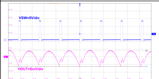
Figure17. ET8121 Output Ripple
