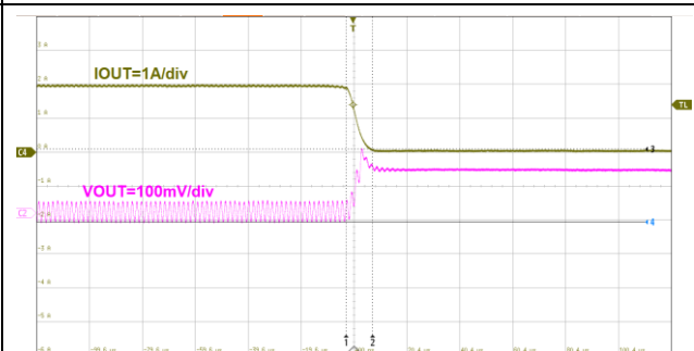
20us/div V_{OUT}=5V I_{OUT}=2A to 0A Figure35. ET8121 Load Transient
