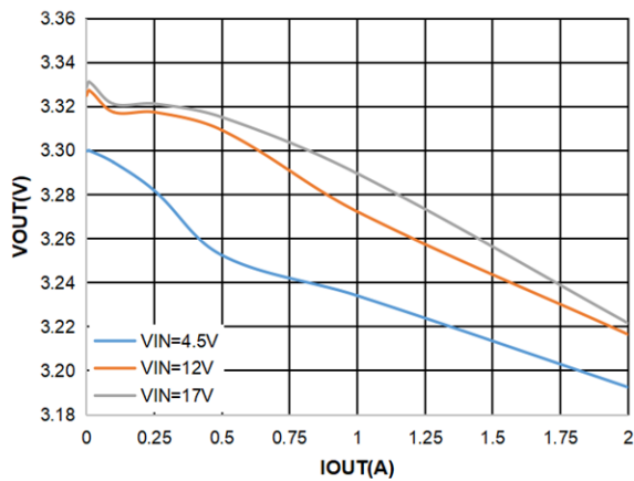
Figure9. ET8121 Load Regulation, V_{OUT}=3.3V
