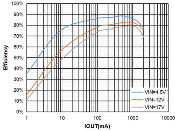
Figure5. V_{OUT}=1.0V Efficiency, L=2.2\mu H
