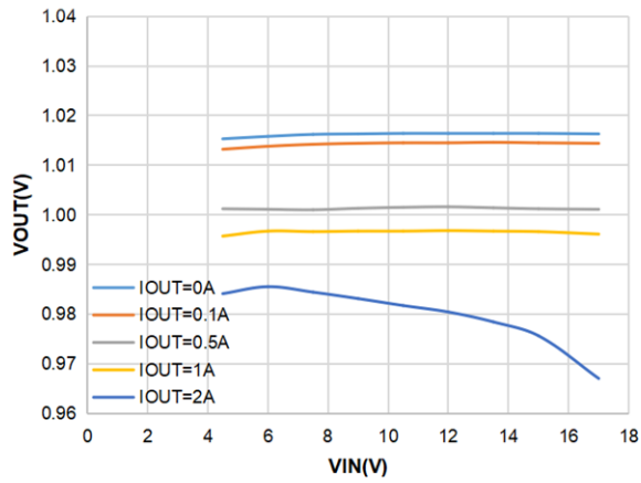
Figure11. ET8121 Line Regulation, V_{OUT}=1.0V
