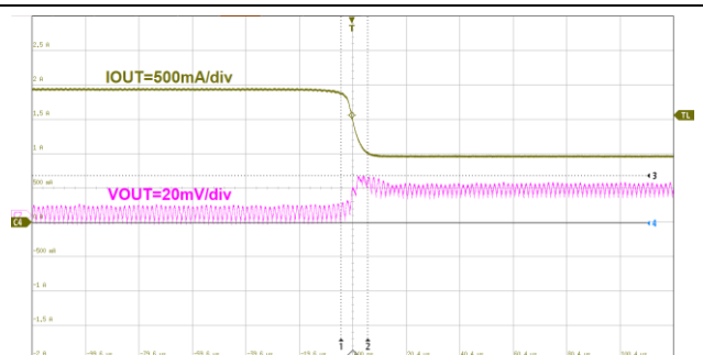
20us/div V_{OUT}=1.0V I_{OUT}=2A to 1A Figure29. ET8121 Load Transient
