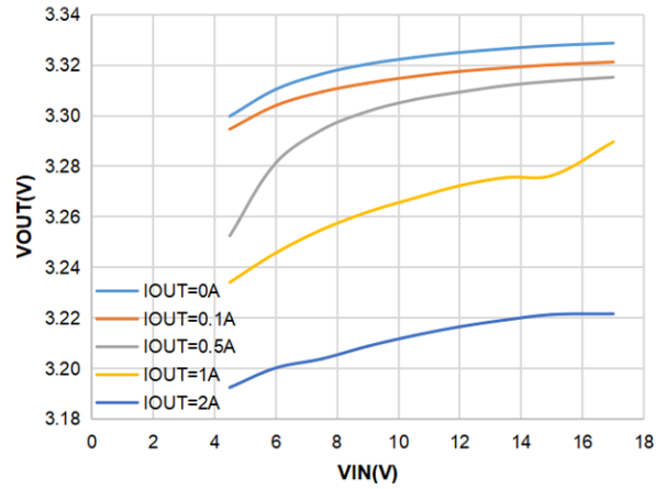
Figure12. ET8121 Line Regulation, V_{OUT}=3.3V
