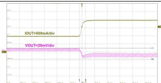
20us/div V_{OUT}=1.0V I_{OUT}=1A to 2A Figure28. ET8121 Load Transient
