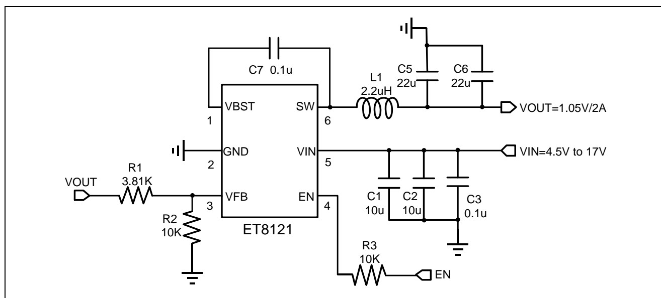
OUT=1.05V/2A Reference Design
