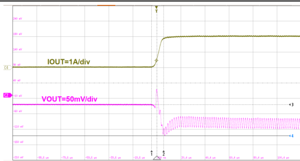
20us/div V_{OUT}=3.3V I_{OUT}=0A to 2A Figure30. ET8121 Load Transient
