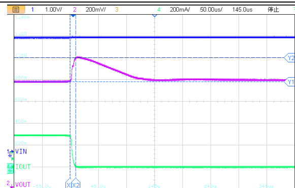
Load Transient(300mA~1mA t=10μs)
