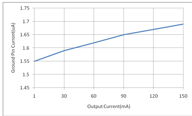
Ground Pin Current VS Output Current
